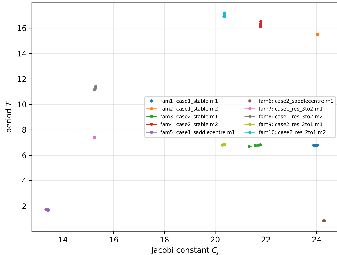
Period vs Jacobi constant along each family
