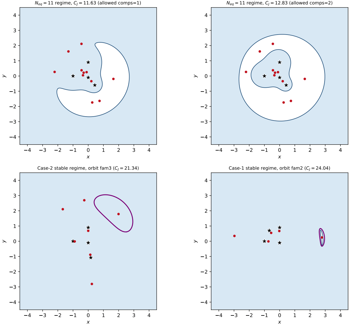
Figure 15: Hill regions (shaded: allowed, 2\Omega \geq C_J ; blue: zero-velocity curve). Stars denote primaries, red points equilibria, and purple curves periodic orbits. Top: the eleven-equilibrium regime at C_J = 11.63 (left) and C_J = 12.83 (right), bracketing a small cluster of finite critical Jacobi levels; the allowed set changes from one connected component to two across this interval as a neck closes. Bottom: representative Floquet-stable periodic orbits in the Case-2 (family 3, left) and Case-1 (family 2, right) regimes, each shown at its own Jacobi constant.
