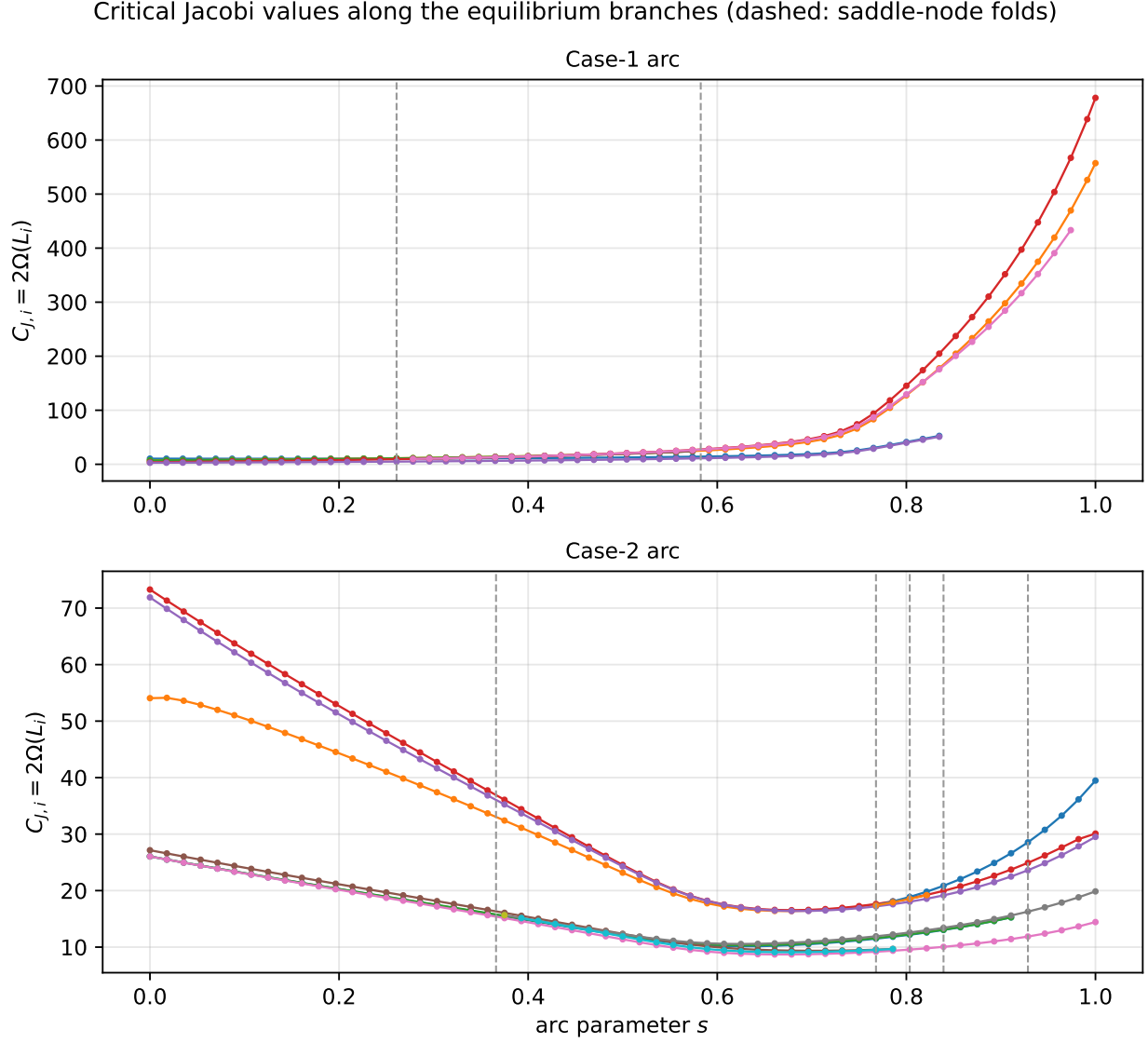
Figure 14: Critical Jacobi values C_{J,i}(s) = 2\Omega(L_i(s)) along the reliably tracked equilibrium branches of the two admissible arcs. Dashed vertical lines mark the saddle-node folds. Each curve gives a finite critical level at which the regular Hill-region topology may change.
