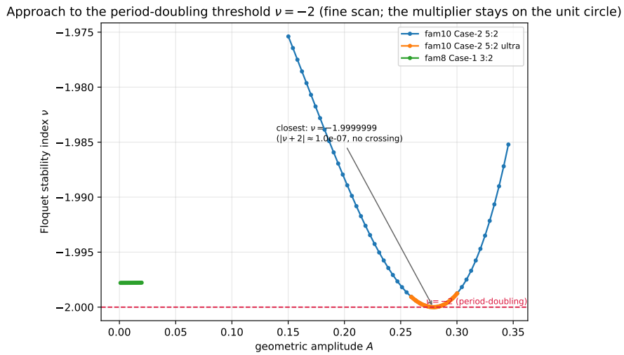
Figure 13: Fine scan of the Floquet index toward \nu = -2 . Family 10 approaches the threshold to within \sim 10^{-7} and returns; the multiplier does not cross -1 . No period-doubling bifurcation occurs.
