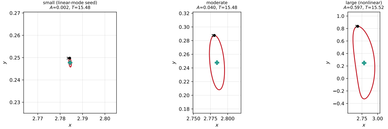
Figure 9: Stable Lyapunov family from the Case-1 arc equilibrium (mode \omega_2 ): small (linear-mode seed), moderate, and large members. Green +: parent equilibrium; black dot: initial point; arrow: direction; stars: primaries in view. Floquet stable throughout.
