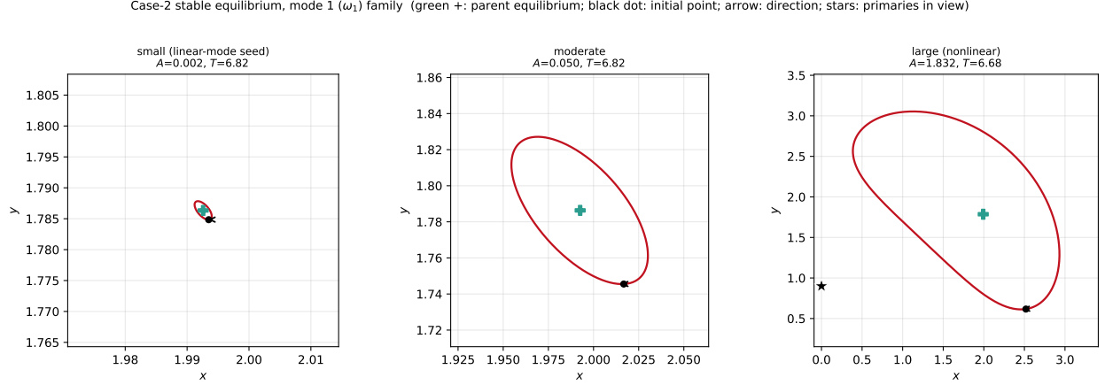
Figure 11: Stable Lyapunov family from the Case-2 arc equilibrium (mode \omega_1 ). Floquet stable throughout.
