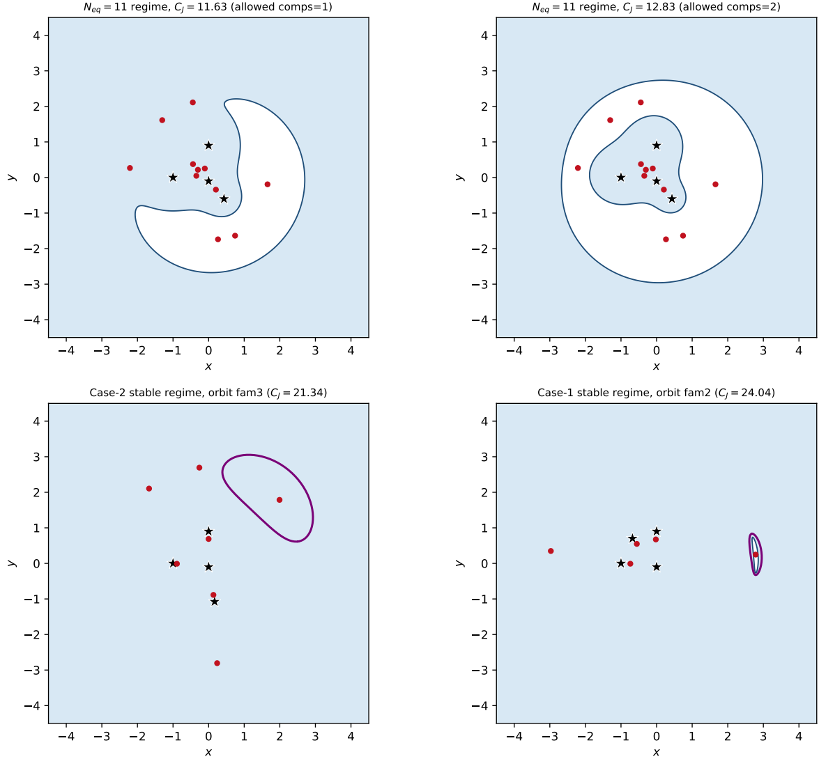
Figure 16: Hill regions (shaded: allowed, 2\Omega \geq C_J ; blue: zero-velocity curve). Stars denote primaries, red points equilibria, and purple curves periodic orbits. Top: the eleven-equilibrium regime at C_J = 11.63 (left) and C_J = 12.83 (right), bracketing a small cluster of finite critical Jacobi levels; the allowed set changes from one connected component to two across this interval as a neck closes. Bottom: representative Floquet-stable periodic orbits in the Case-2 (family 3, left) and Case-1 (family 2, right) regimes, each shown at its own Jacobi constant.
