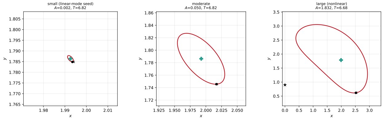
Figure 11: Stable Lyapunov family from the Case-2 arc equilibrium (mode \omega_1 ). Floquet stable throughout.
