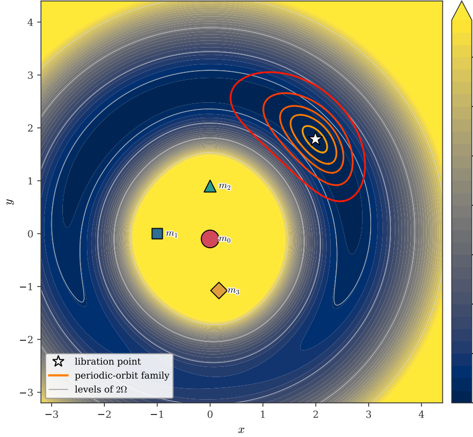
Figure 9: Effective-potential landscape for the Case-2 configuration supporting periodic-orbit family 3. Filled contours show 2\Omega(x, y) , with the colour range clipped at large values for visualization; 2\Omega \rightarrow +\infty at the primary singularities and at large distance. Thin grey curves are representative level curves of 2\Omega at 22.29, 23.29, 25.29, and 28.79. The four primaries are marked by m_0 – m_3 , and the star denotes the doubly-elliptic parent equilibrium. The Hessian of \Omega at this point has eigenvalues 0.0436 and 2.9554, so the parent is a strict local minimum of the effective potential. Successive members of the associated Lyapunov family are shown from small to larger amplitude, illustrating libration about the equilibrium of the rotating four-primary configuration rather than orbital motion about any individual primary.
