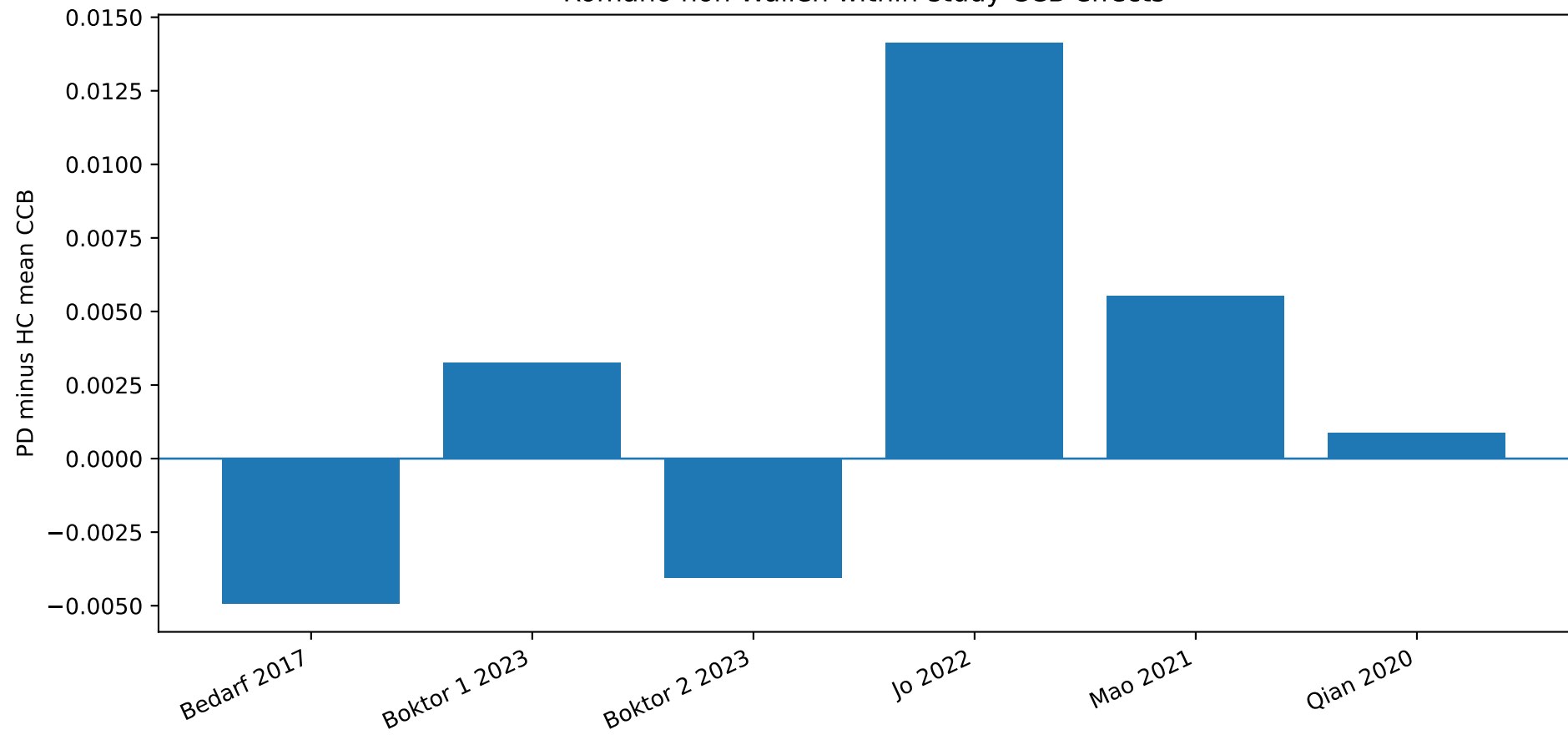
Romano non-Wallen within-study CCB effects
