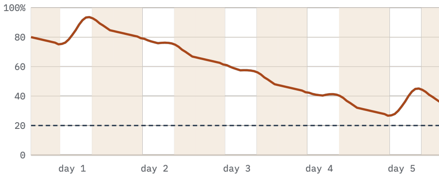
Figure 3.1. State of charge of the 5.1 kWh bank over five December days: clear, three overcast, clear. Shaded: night. Dashed: the 20% floor.
