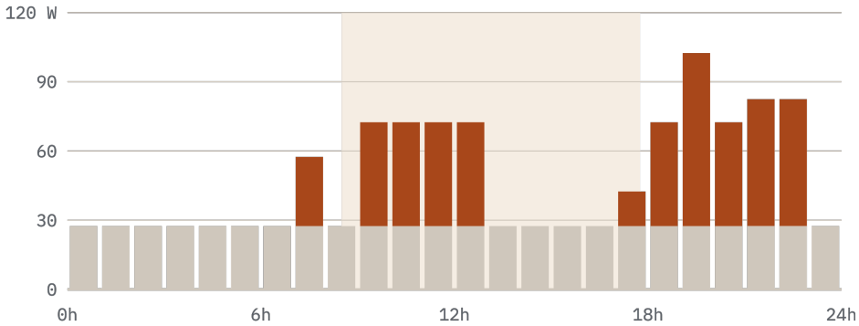
Figure 1.1. Average draw, hour by hour, on a winter day. Grey: the constant floor of fridge, router and inverter; orange: everything else; pale band: daylight.
