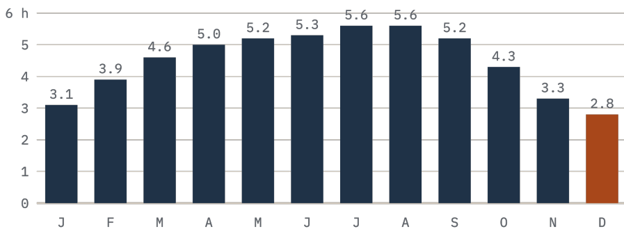
Figure 2.1. Peak sun hours a day by month at 42° N, panels tilted at 60°. December is the design month.
