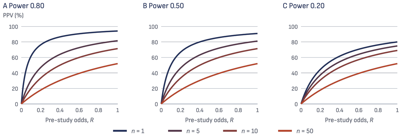
Figure 2. PPV (Probability That a Research Finding Is True) as a Function of the Pre-Study Odds for Various Numbers of Conducted Studies, n . Panels correspond to power of 0.80, 0.50, and 0.20. Drawn in code from Eq. (3).
