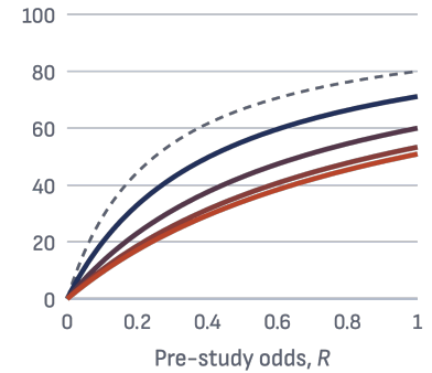
Figure 1. PPV (Probability That a Research Finding Is True) as a Function of the Pre-Study Odds for Various Levels of Bias, u
