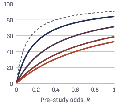
Figure 1. PPV (Probability That a Research Finding Is True) as a Function of the Pre-Study Odds for Various Levels of Bias, u
