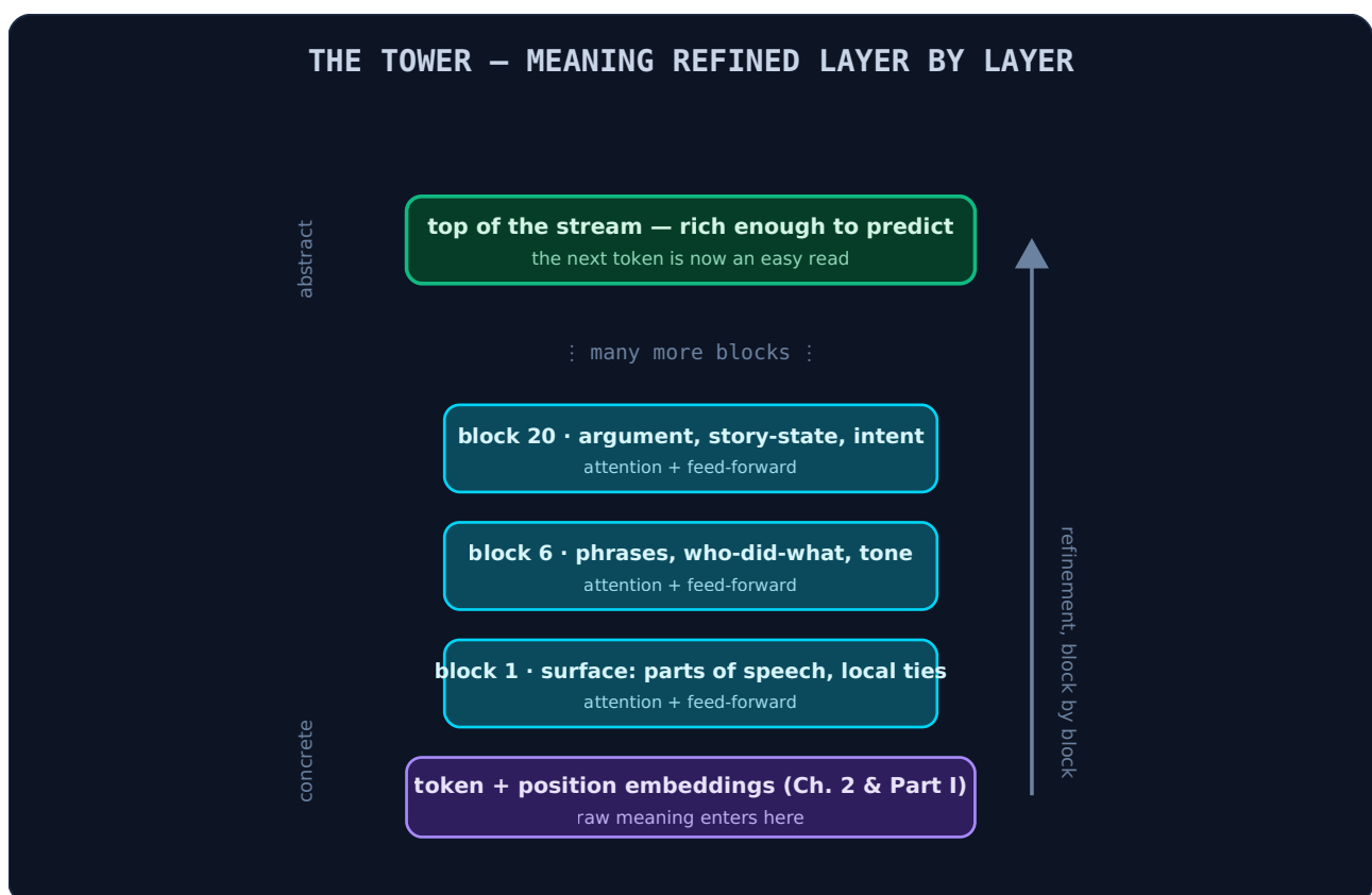
Figure 4. Depth as refinement. The same token vector rises through the stack, each block adding a slightly more abstract reading. The labels here are a useful cartoon, not a precise map — the division of labour across real layers is blurrier and is still being charted by interpretability research — but the direction of travel is real: concrete near the bottom, abstract near the top. Depth is not repetition; it is elaboration.
