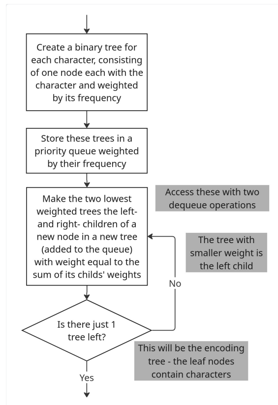
Figure 4: A flowchart depicting the creation of the Huffman tree
