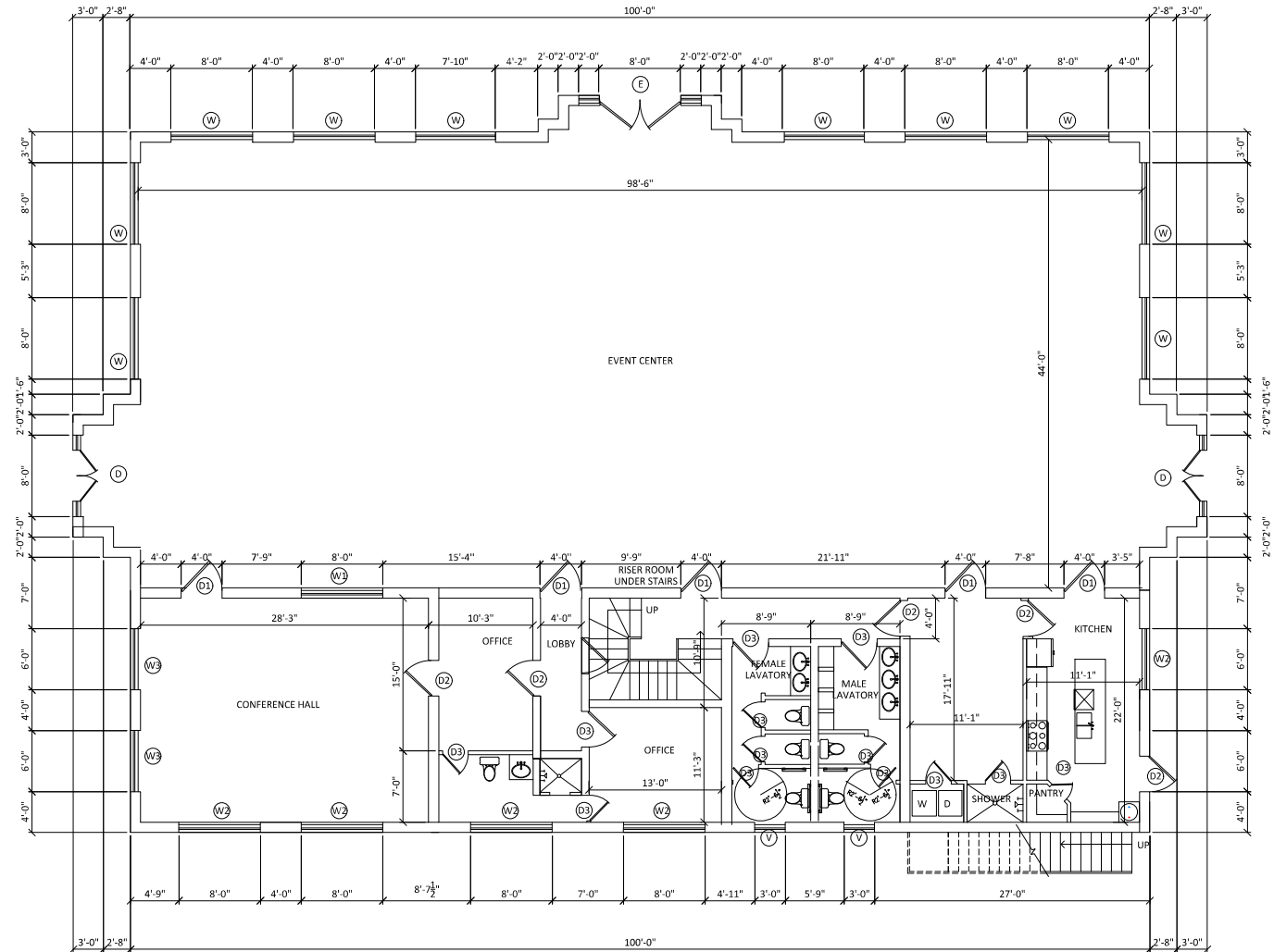
① FIRST FLOOR PLAN
