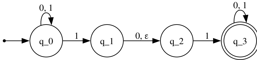
Figure 1: graphs/02_nfa.gv
