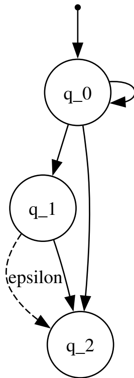
Figure 2: graphs/02_tree.gv
