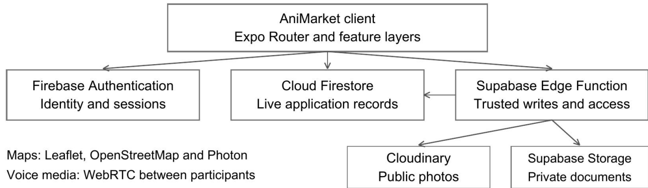
Figure 1 AniMarket system architecture
