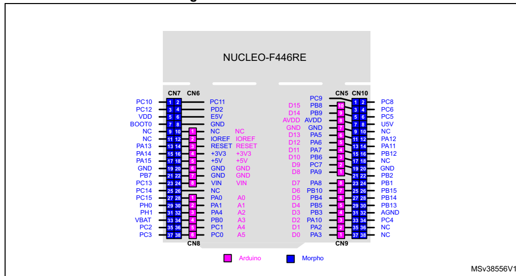
Figure 25. NUCLEO-F446RE
