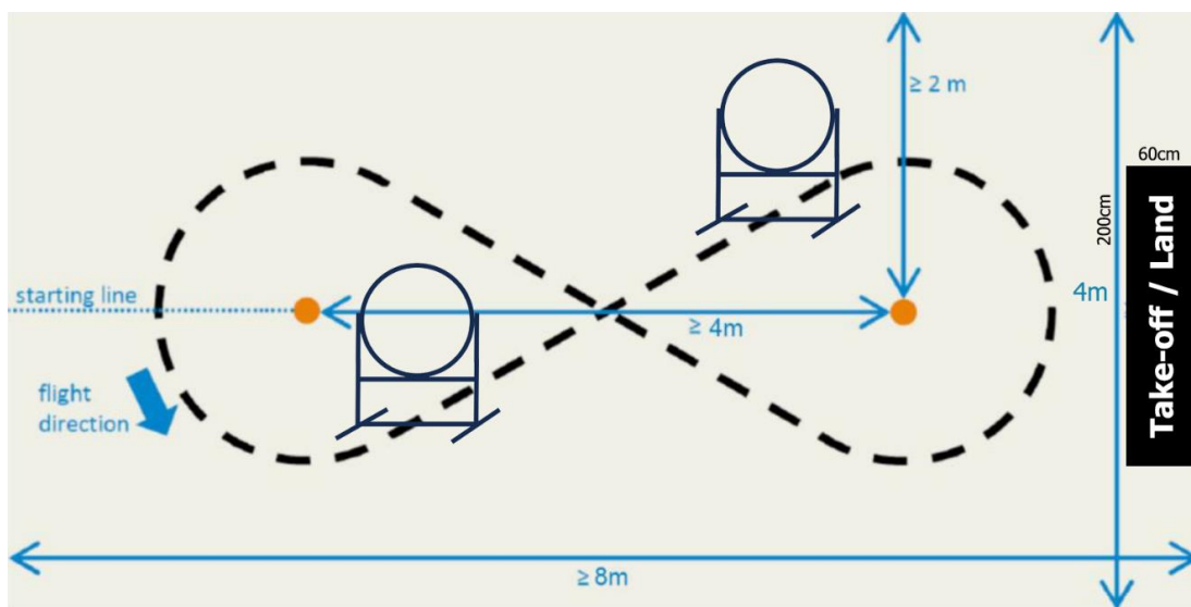
Top View of the Competition Field and Flight Path
