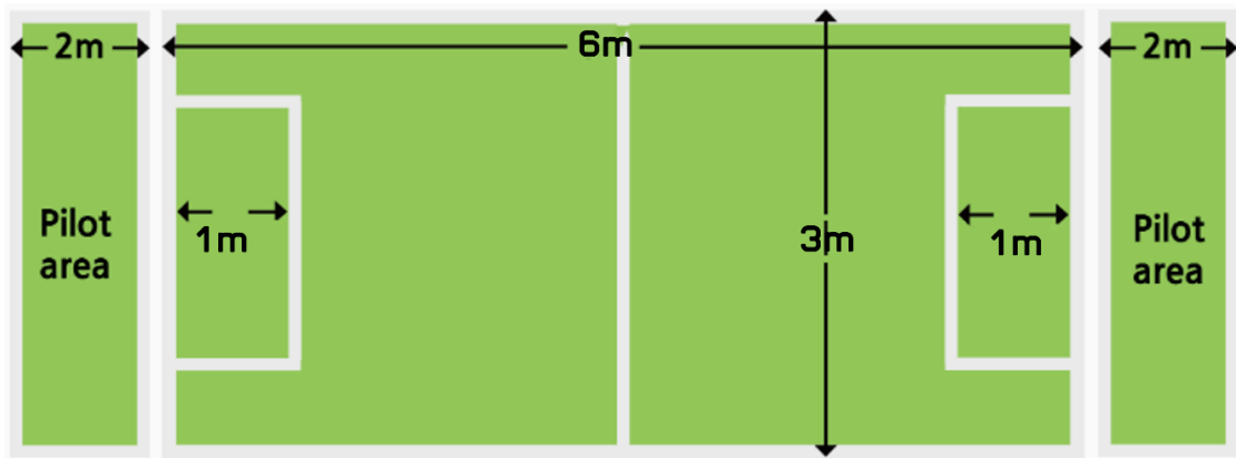
Top View of the Competition Field
