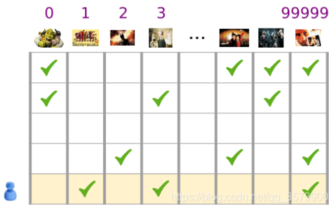
Figure 3. Data for our movie recommendation problem.
