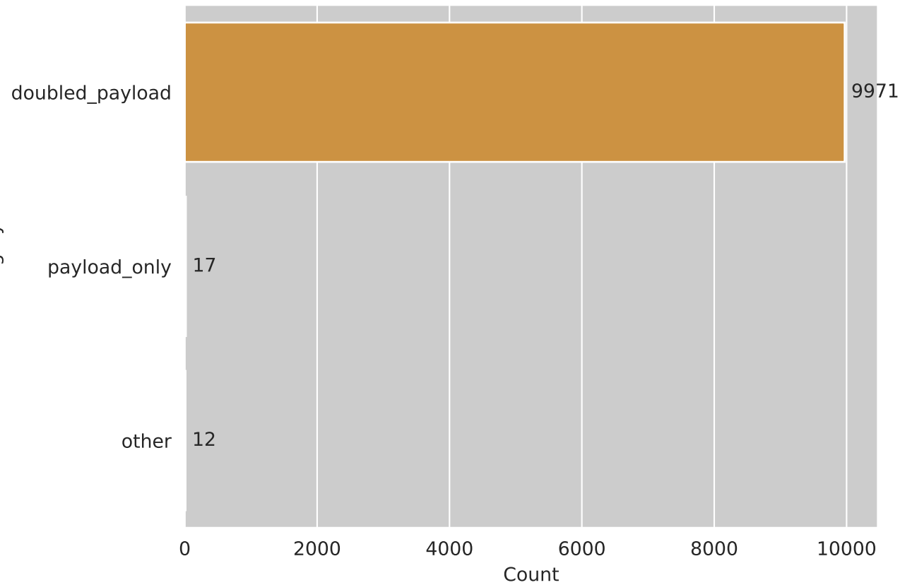
Sequence Counts
