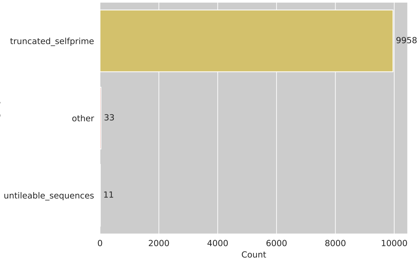
Sequence Counts
