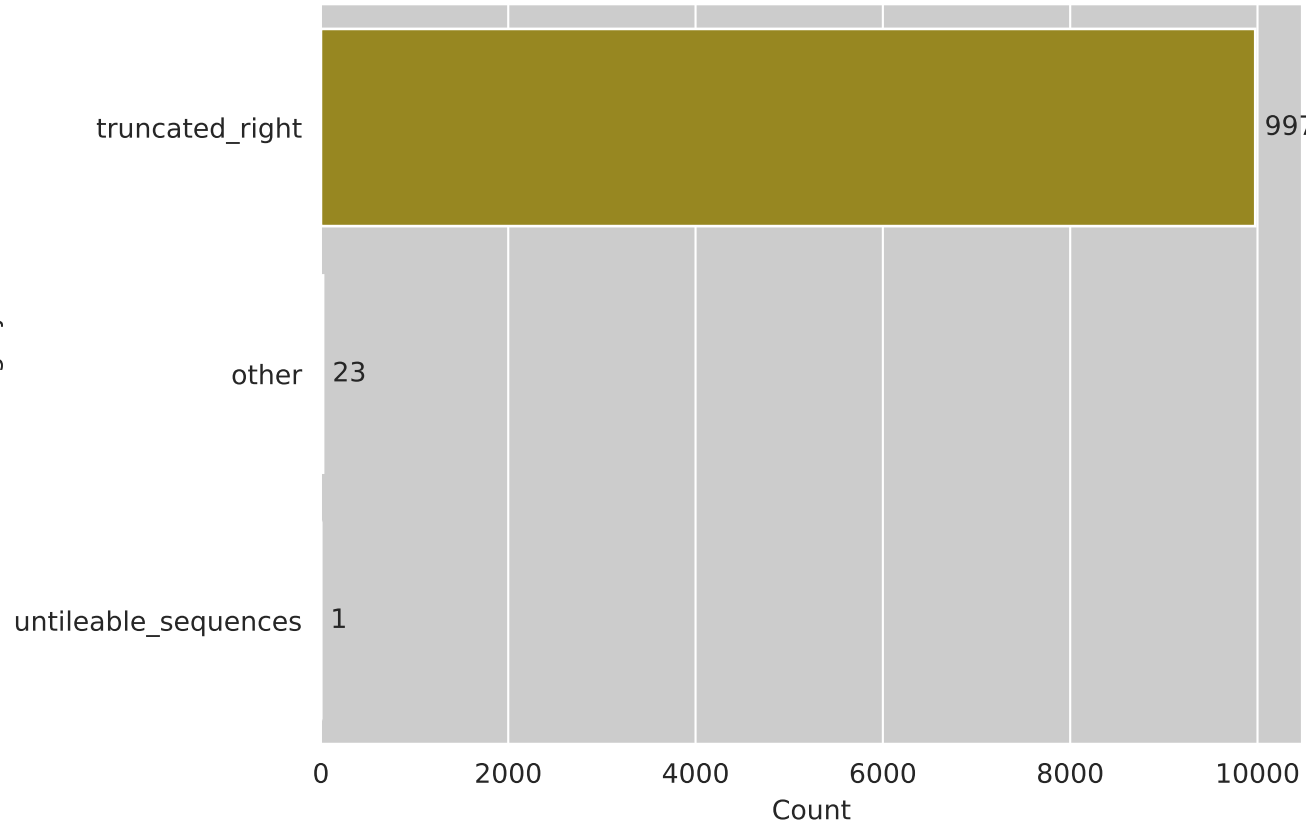
Sequence Counts
