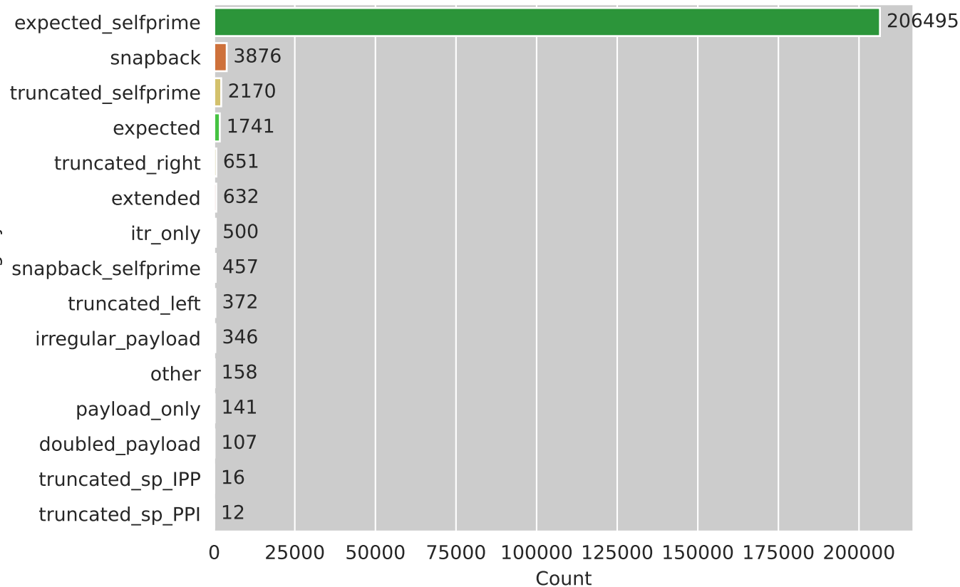
Sequence Counts
