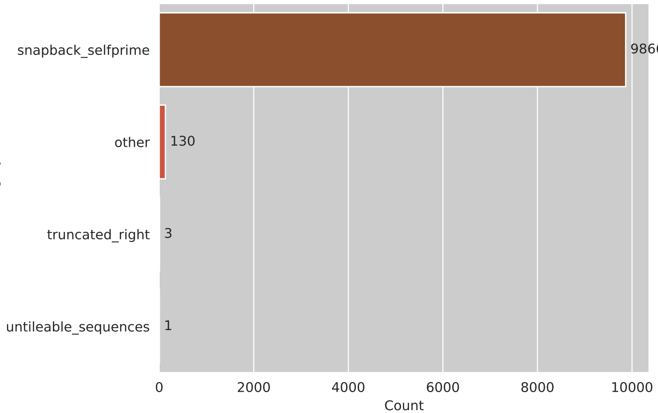
Sequence Counts
