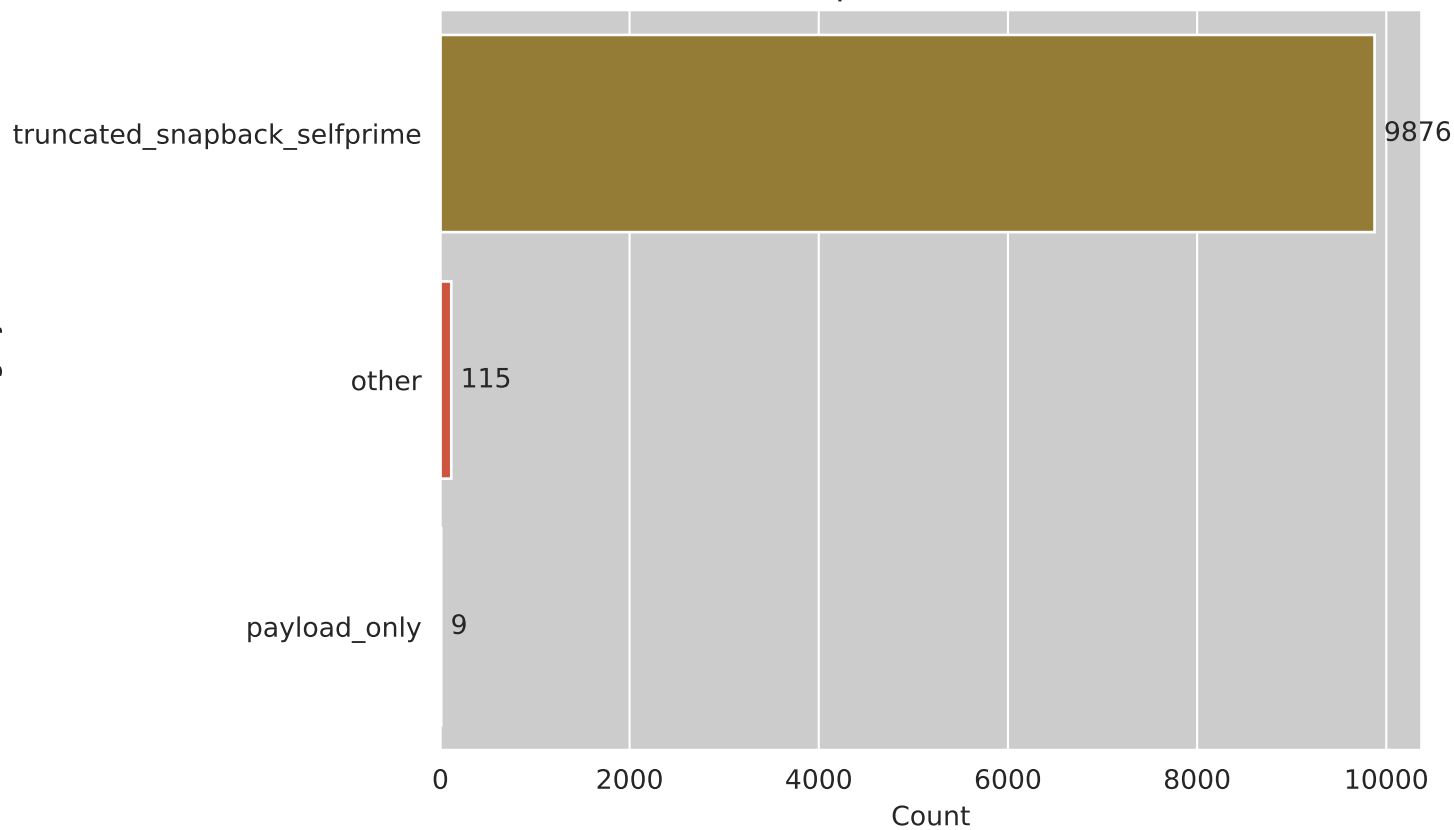
Sequence Counts
