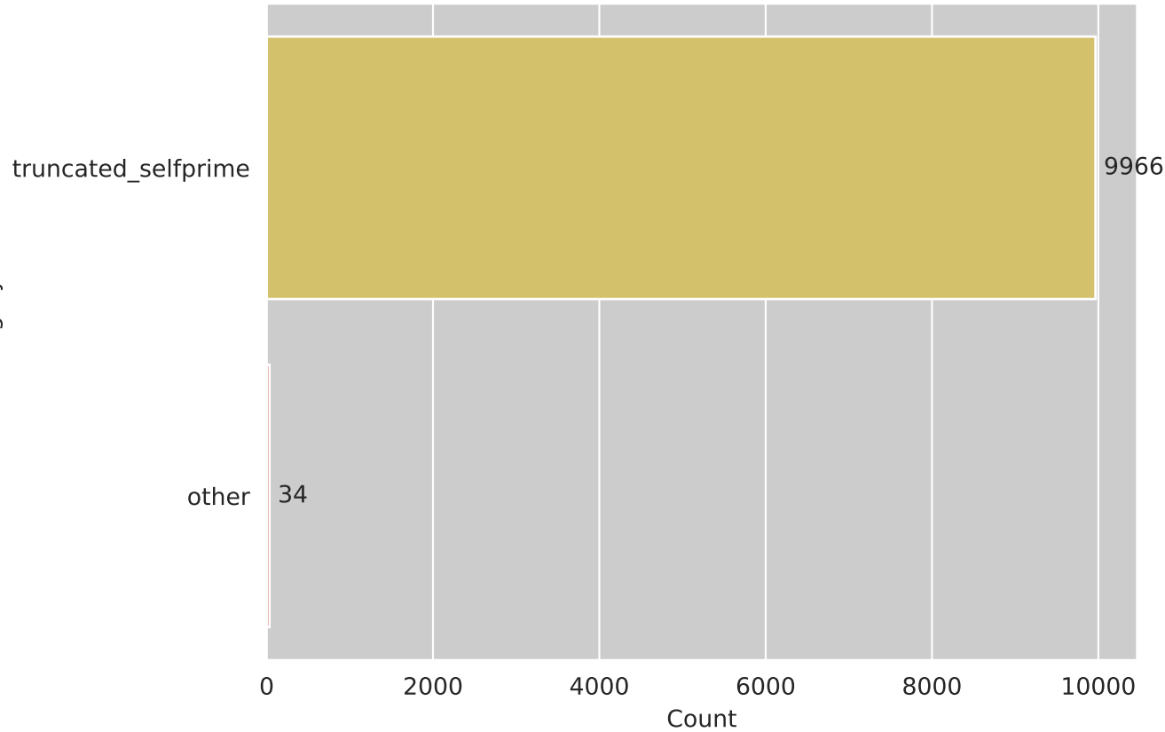
Sequence Counts
