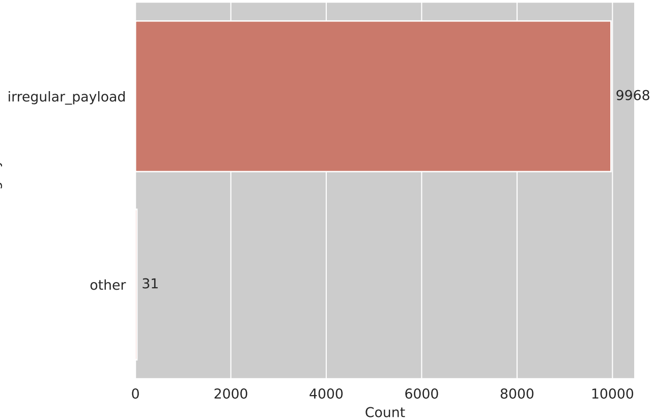
Sequence Counts
