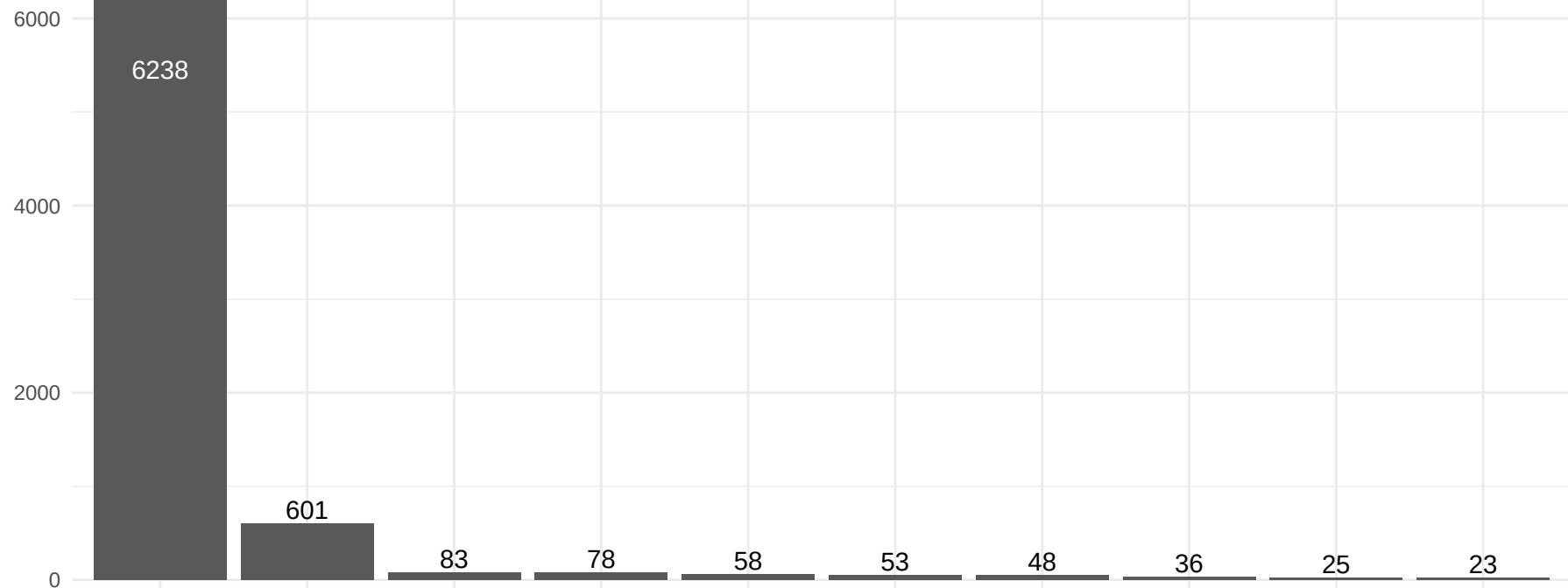
Protein detection overlap across conditions
