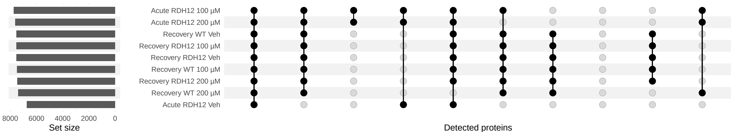
Protein detection overlap across conditions
