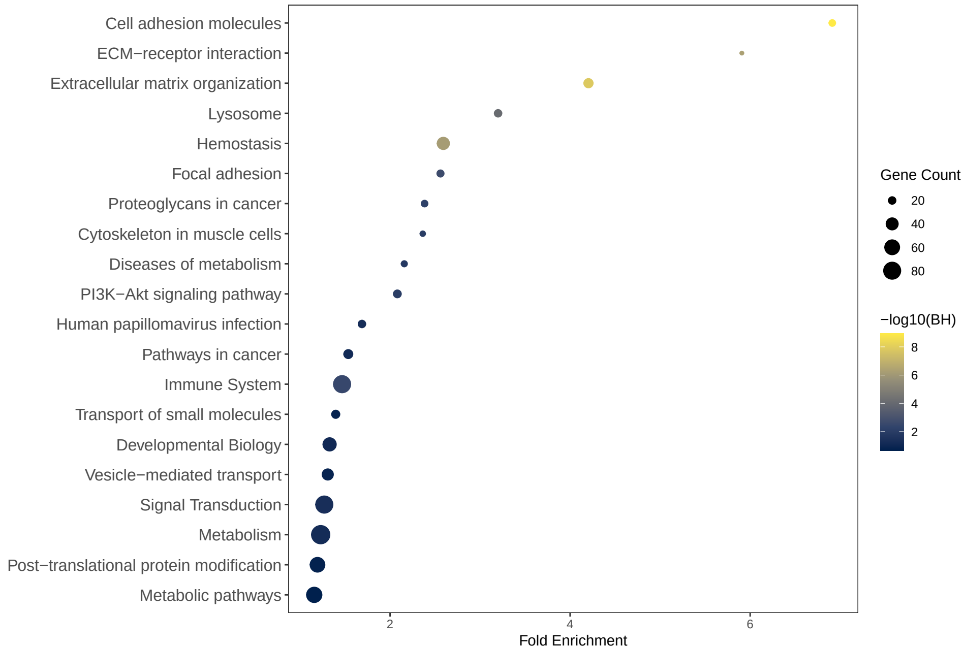
Top Nonredundant Enriched Pathways (BH ≤ 0.25)
