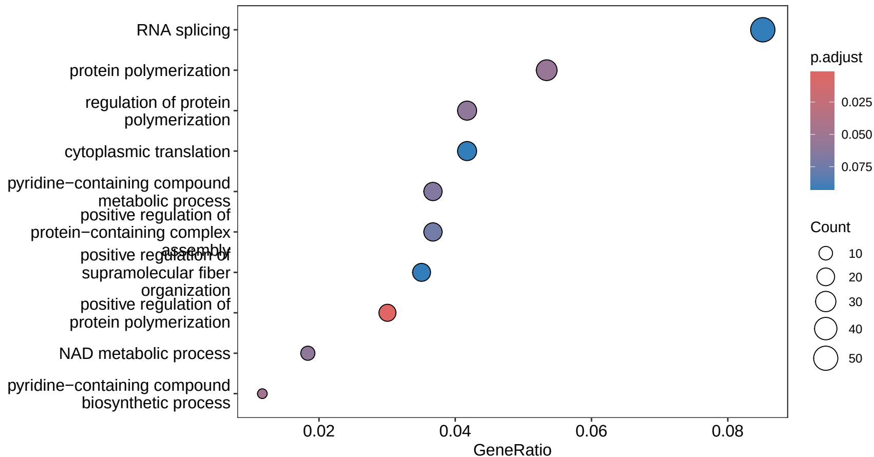
shared_down_100uM_200uM: GO BP (simplified)
