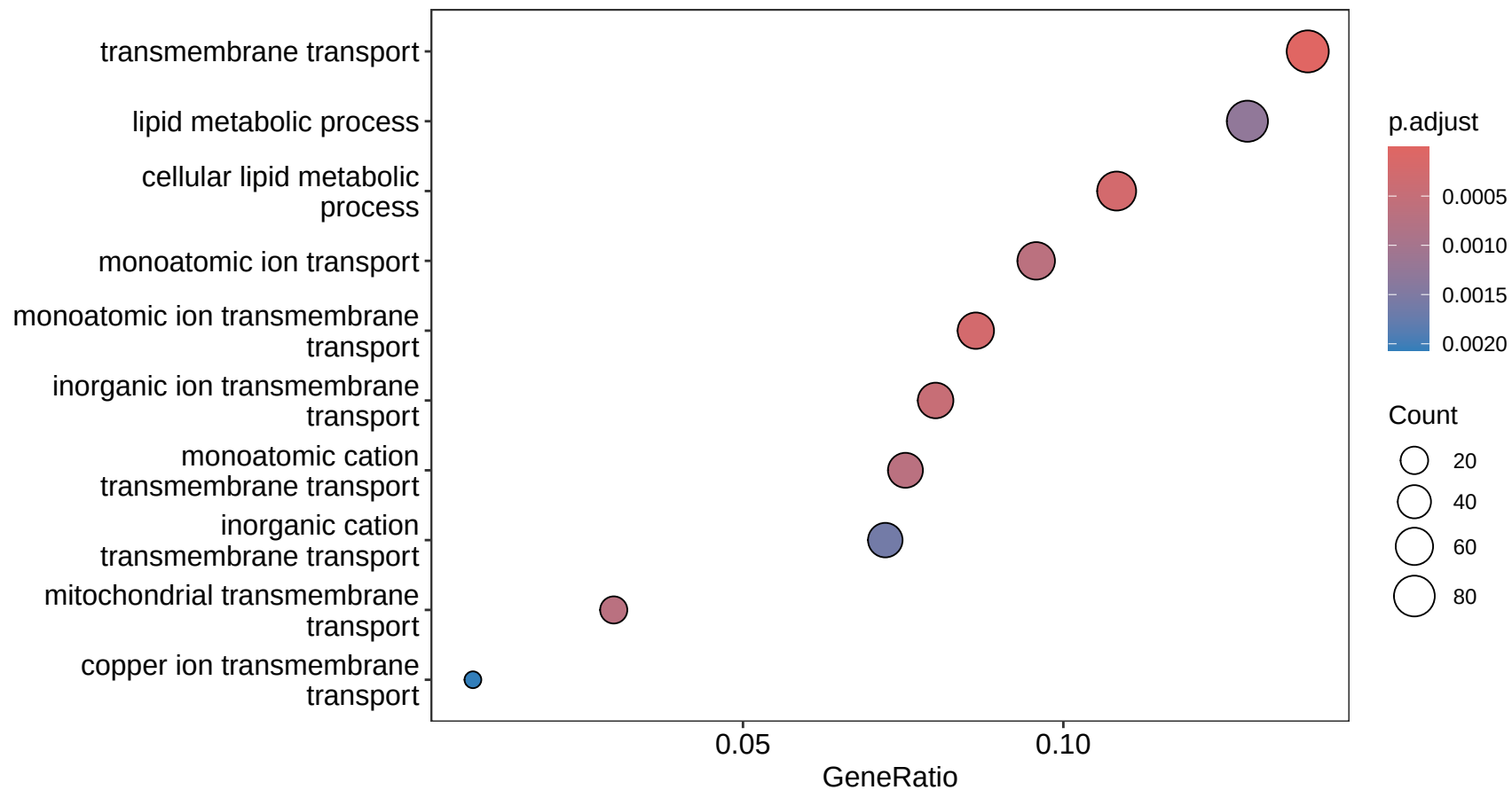
RDH12_200_atRAL5hr_vs_RDH12_control_atRAL5hr_up: GO BP (simplified)
