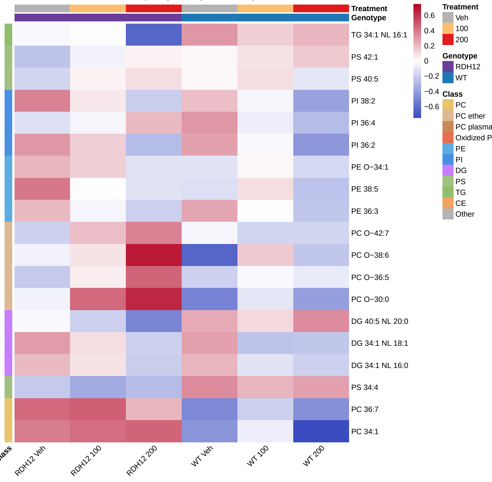
Recovery targeted lipid heatmap
