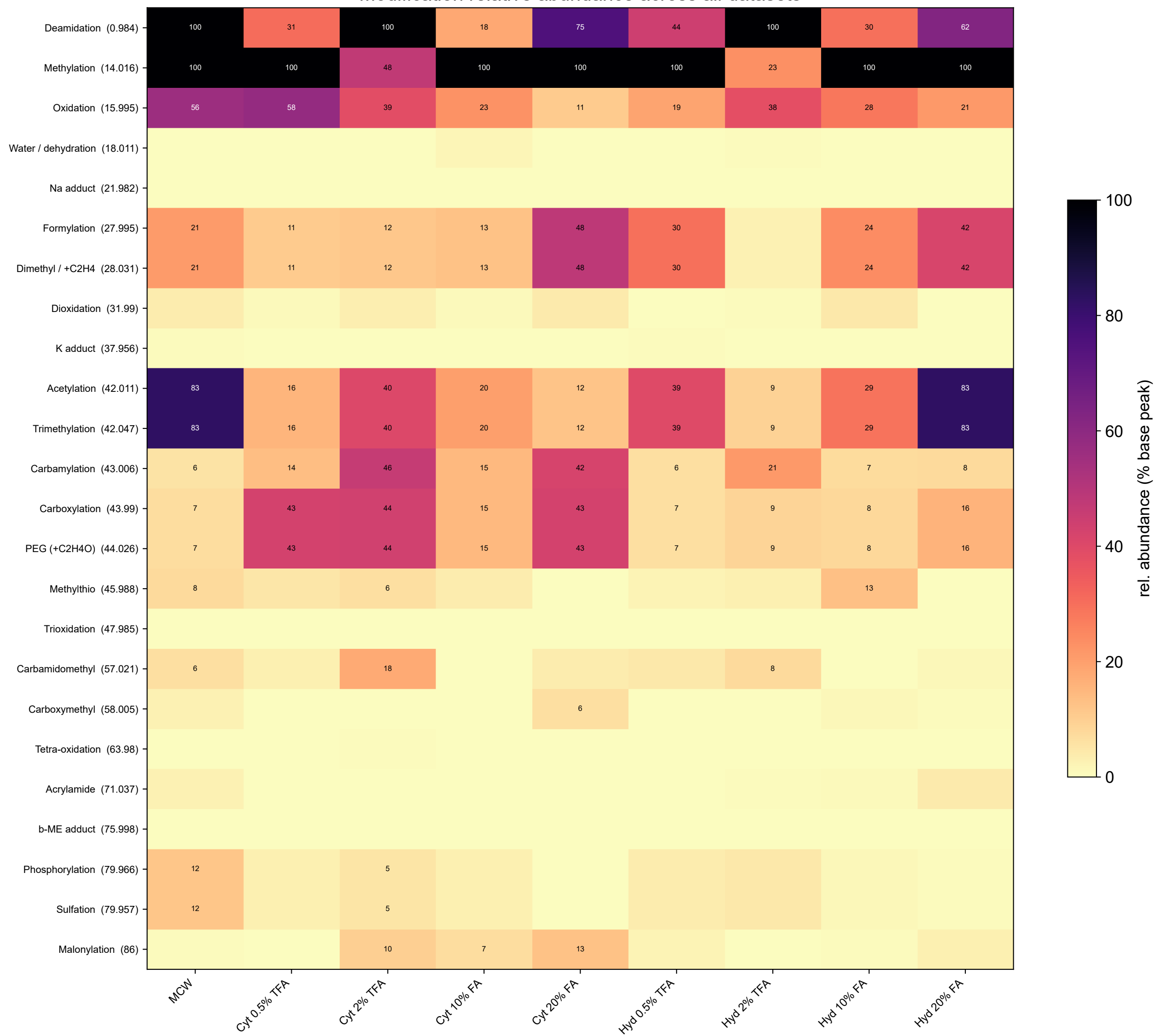
Modification relative abundance across all datasets
