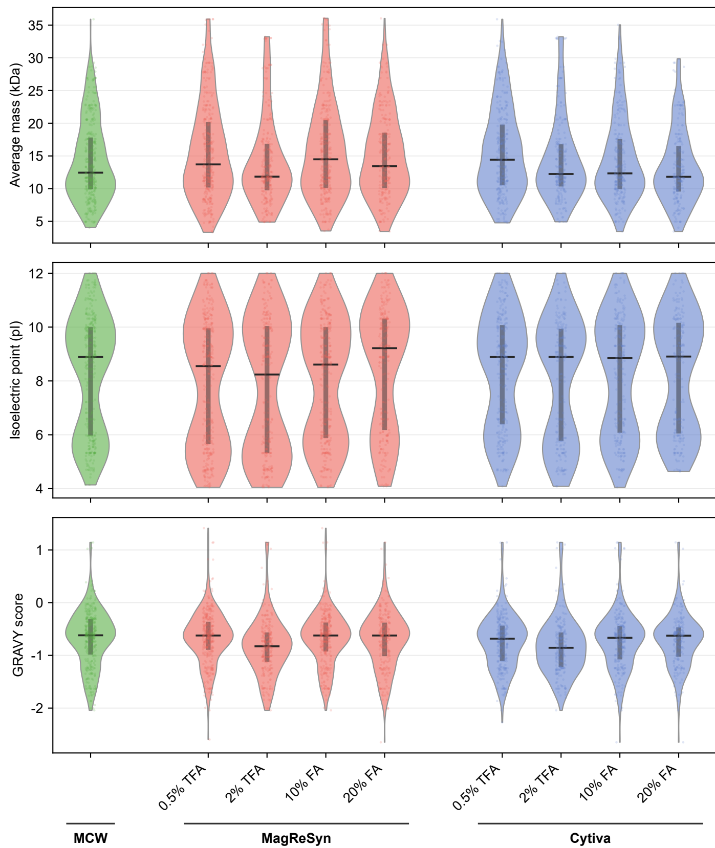
Proteome physicochemical properties by condition, histones excluded (n=698 proteoforms)
