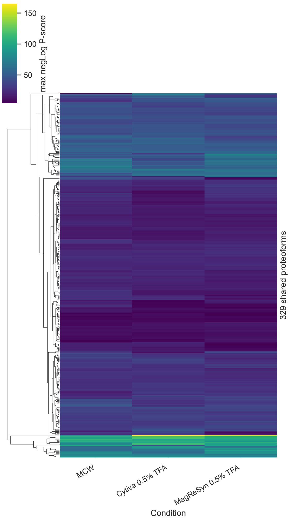
Shared proteoforms: negLog P-score by condition
