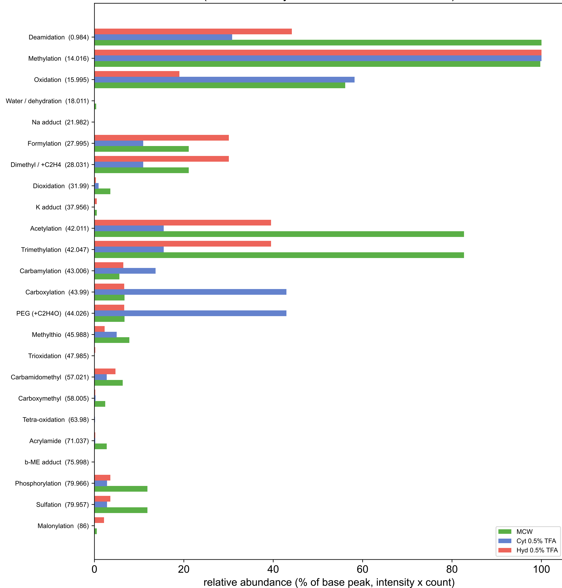
Common modification abundance by cleanup condition (tallest intensity x count bin within +/-0.05 Da)
