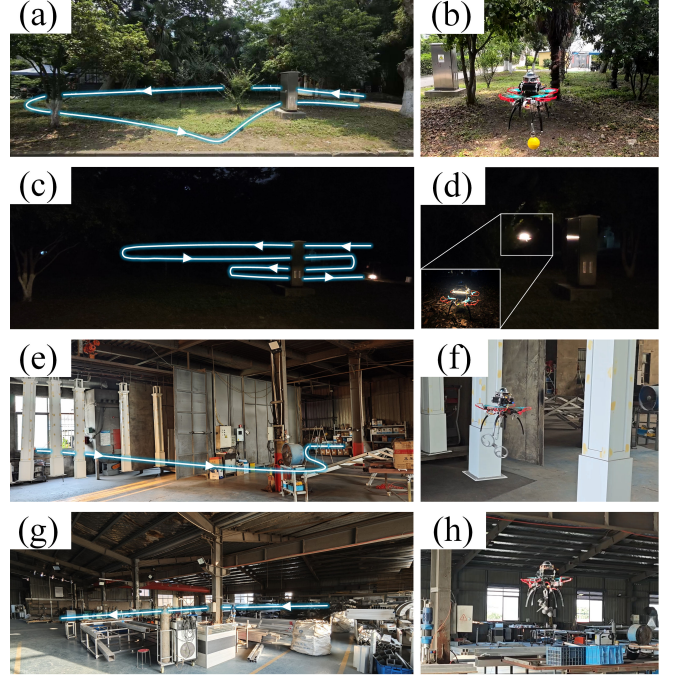
Fig. 1: Disturbance-resilient navigation in cluttered environments. (a)–(d) Flight routes and snapshots in the same wooded scene during daytime and nighttime; (e)–(h) flight routes and snapshots in two factory scenarios.
