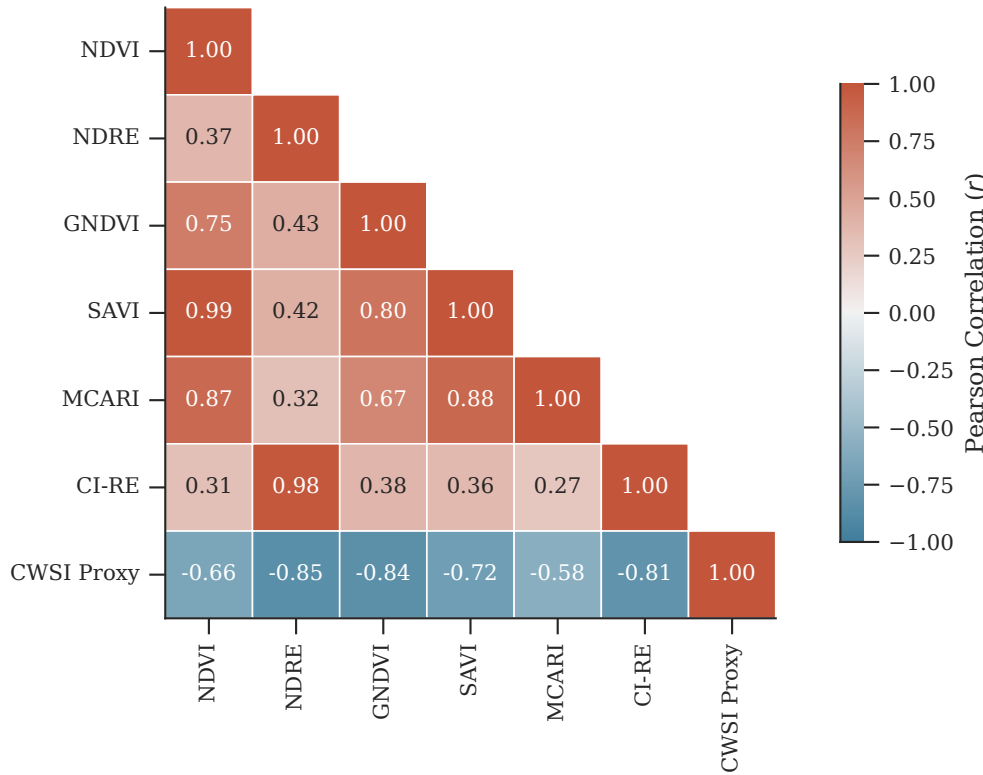
Inter-Index Collinearity Matrix on D1 Potato Dataset (SHAP Baseline)
