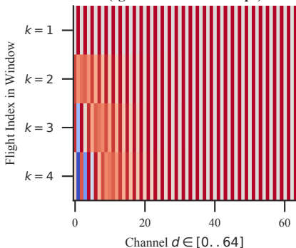
(b) Fixed Discrete Encoding (Ignores Real Time Gaps)
