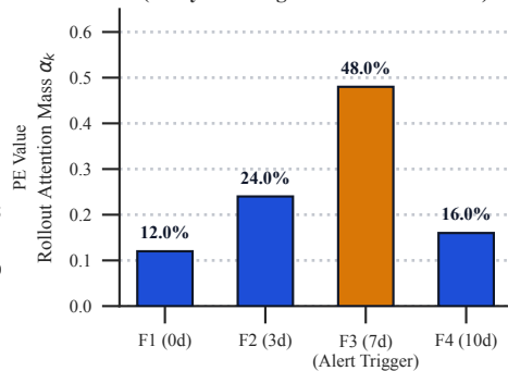
(d) [TREND] Token Attention Rollout (Early Warning Driver Identification)
