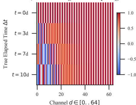
(c) Proposed CTPE( \Delta t ) (Preserves Irregular Time Spacing)
