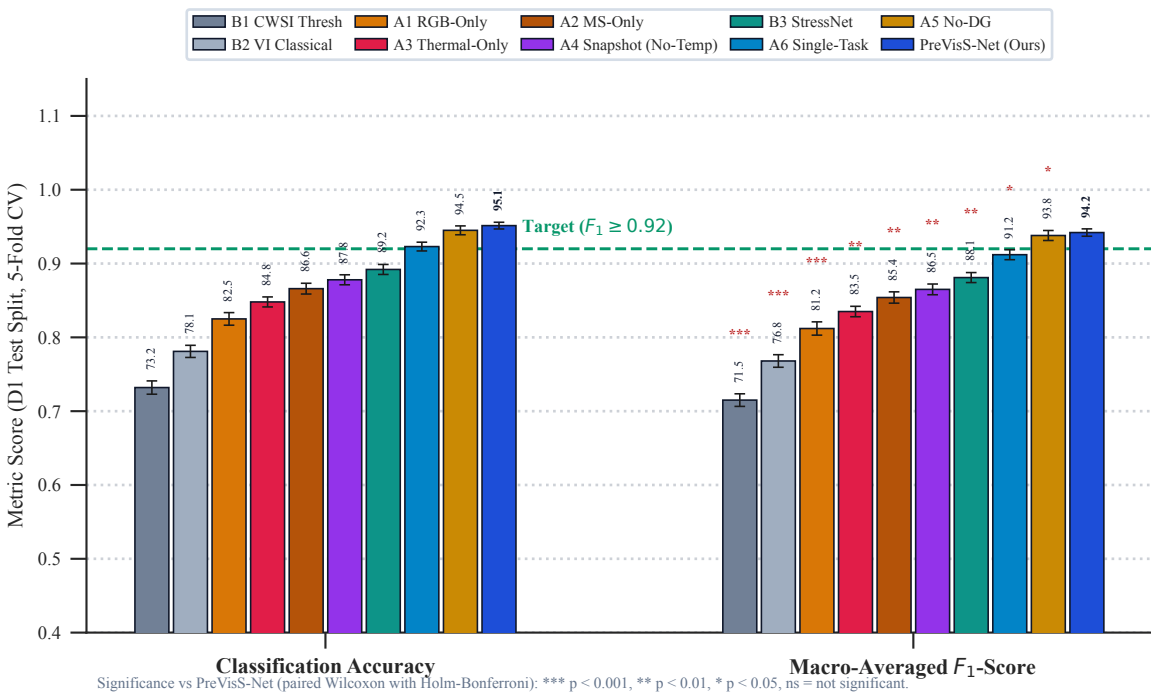
Same-Domain Water-Stress Performance Across 10 Evaluated Methods (Ordered Worst-to-Best)
