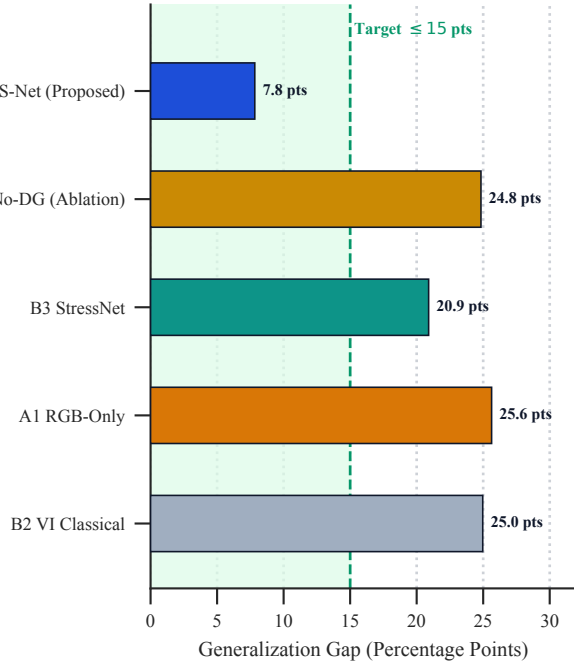
(b) Generalization Gap & Target Check
