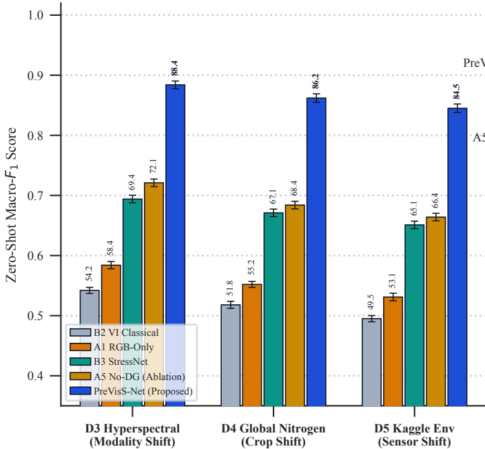
(a) Zero-Shot Out-of-Distribution Transfer
