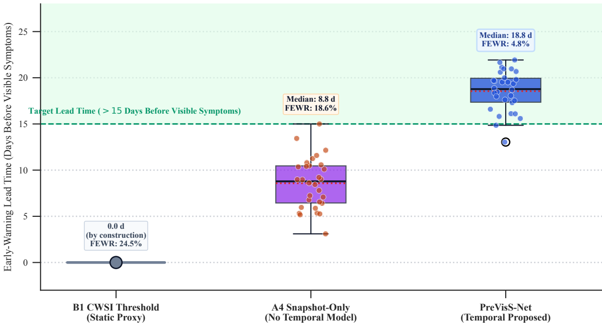
Pre-Visual Early-Warning Lead-Time Distribution on Staged D3 Hyperspectral Dataset
