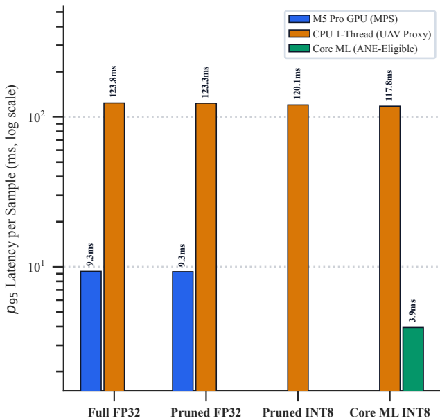
(a) Inference Latency by Hardware Tier
