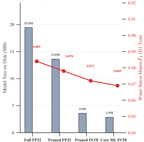
(b) Accuracy vs Model Size Trade-Off
