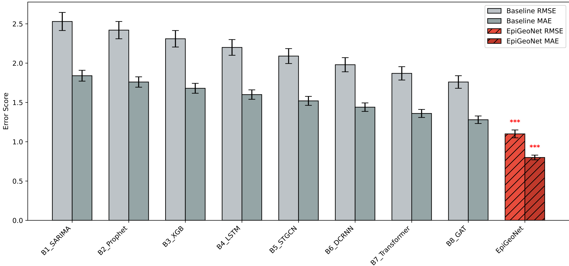
Forecasting Performance across Methods (Worst to Best)
