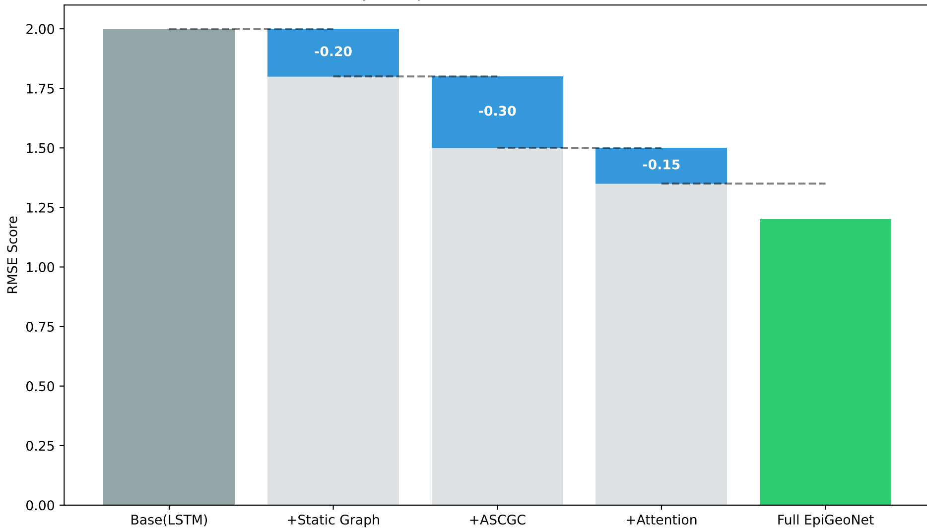
Ablation Study: Component Contributions to RMSE Reduction
