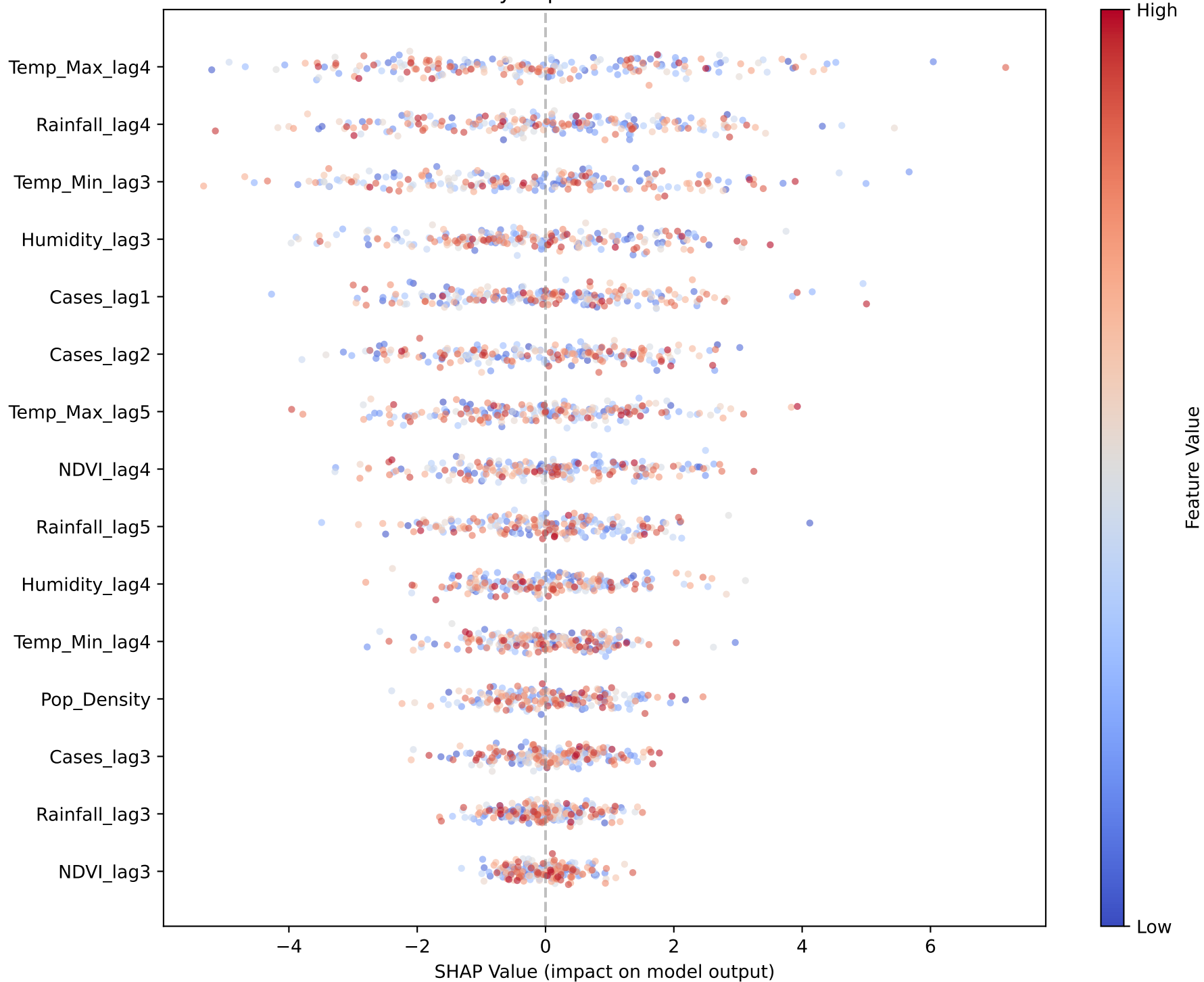
SHAP Summary: Top 15 Drivers of Outbreak Risk
