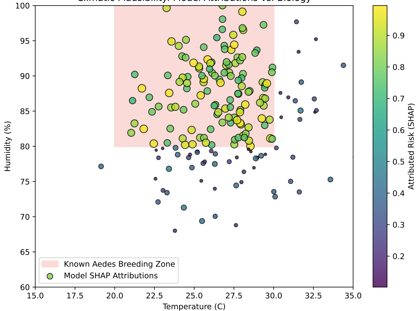
Climatic Plausibility: Model Attributions vs. Biology
