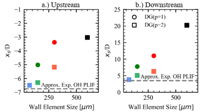
FIG. 12. a.) Upstream and b.) downstream flame stabilization points for each polynomial and grid size
