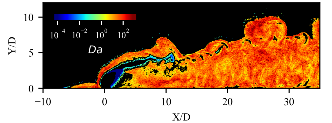
FIG. 17. Instantaneous Damkohler number distribution filtered by the local heat release rate along the centerplane.
