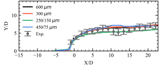
FIG. 11. Mean OH layer location for DG( p=2 ) simulations on each grid size
