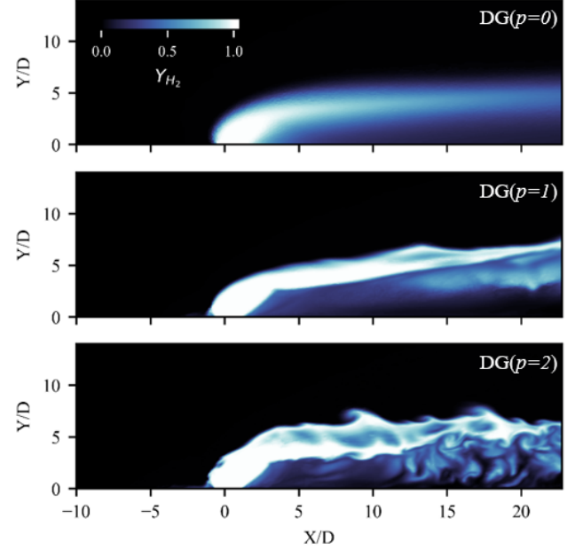
FIG. 5. Centerline contour of Y_{H_2} mass fraction on the 300 \mu\text{m} grid for each polynomial level
