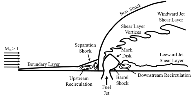
FIG. 2. Centerline schematic diagram of primary flow features present in a transverse jet in supersonic crossflow
