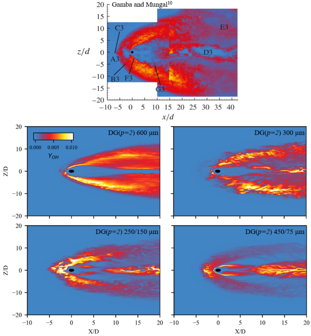
FIG. 14. Experimental instantaneous OH-PLIF image at Y/D = 0.25 from Gamba and Mungal 10 and instantaneous XZ contours of OH mass fraction at Y/D = 0.25 for DG( p = 2 ) solutions on grids with h = 600, 300, 250/150 , and 450/75 \mu\text{m} at the wall.
