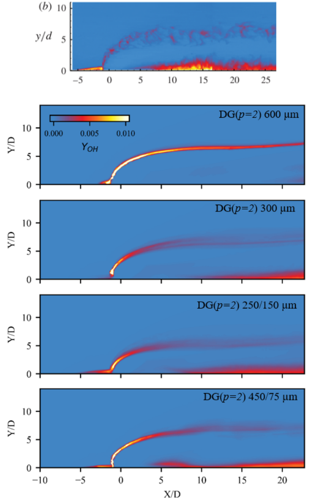
FIG. 9. Experimental centerline average OH-PLIF image from Gamba and Mungal 10 and average centerline contours of Y_{OH} mass fraction for DG(p=2) solution on grids with h = 600, 300, 250/150 , and 450/75 \mu\text{m} at the wall.
