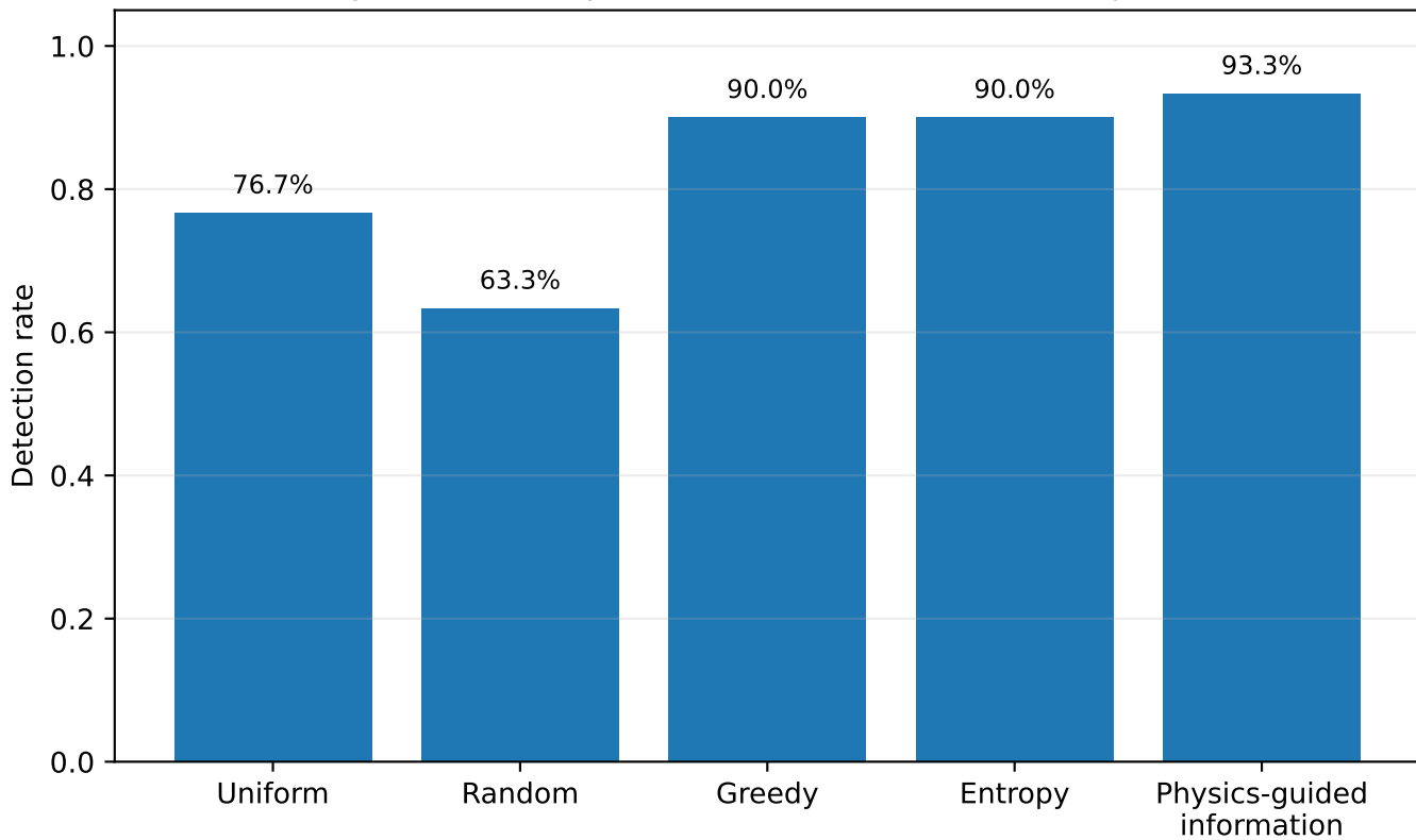
Target-detection performance across allocation policies
