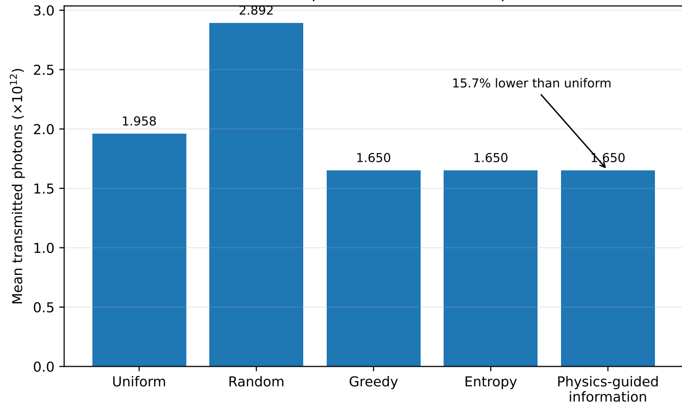
Photon consumption across allocation policies
