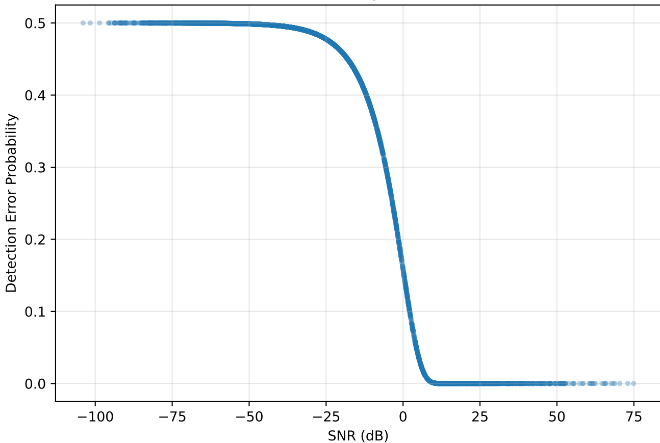
Radar Detection Error Under Noisy Defense Channel Conditions
