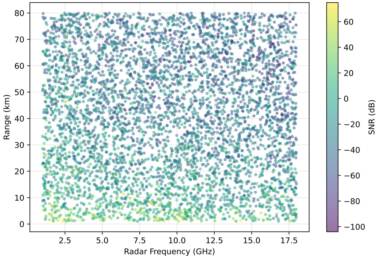
Physics-Based SNR Variation Across Frequency and Range
