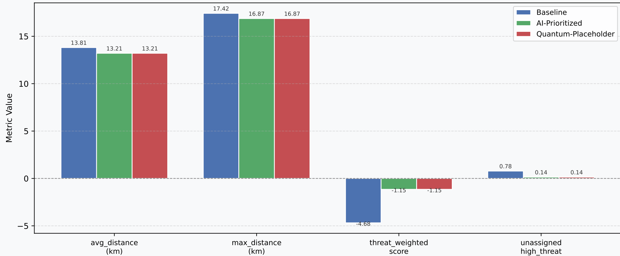
Figure 2: Aggregate Results over 50 Simulation Runs (N=5 attackers, M=3 defenders)
