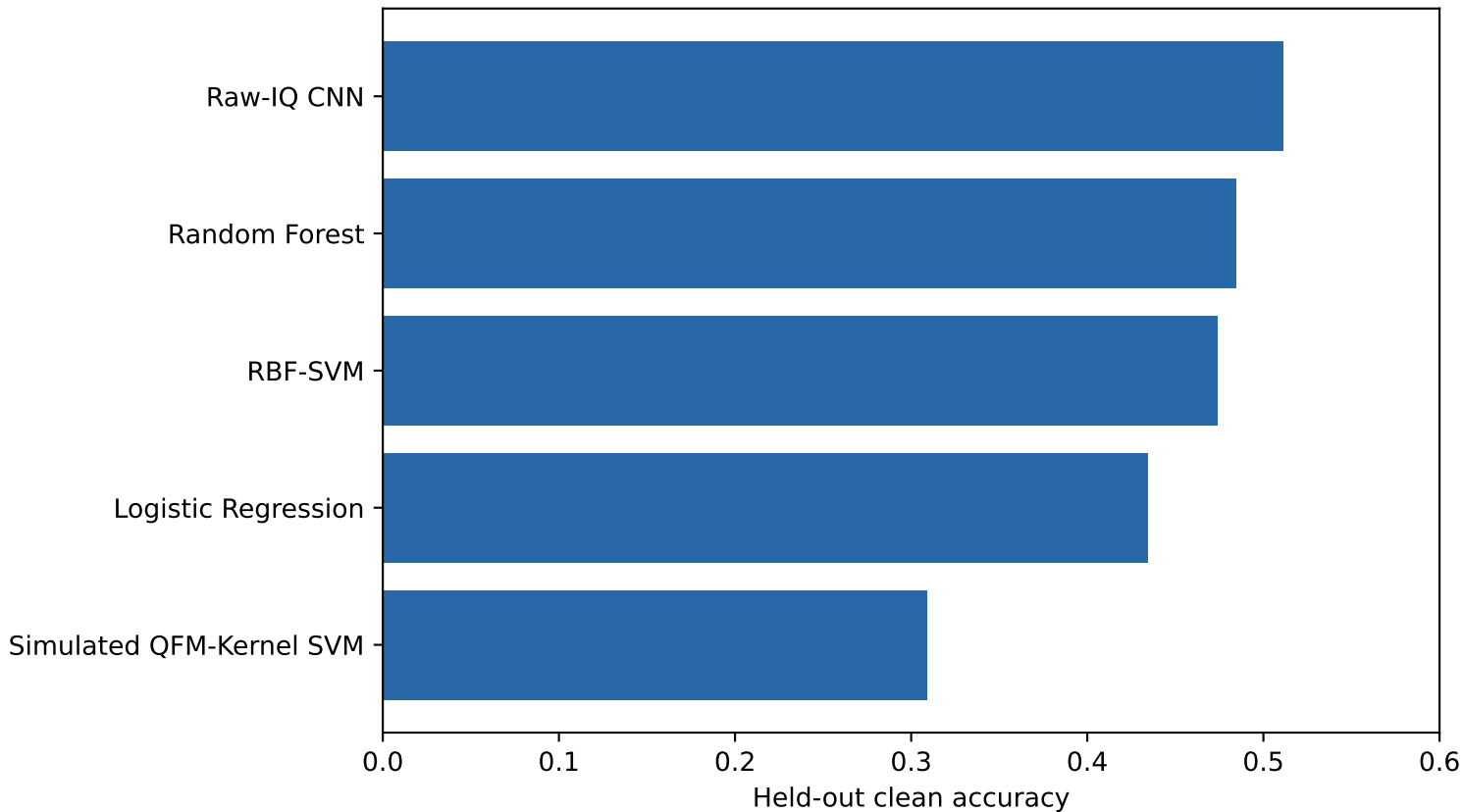
RadioML2016.10A clean-set classification performance
