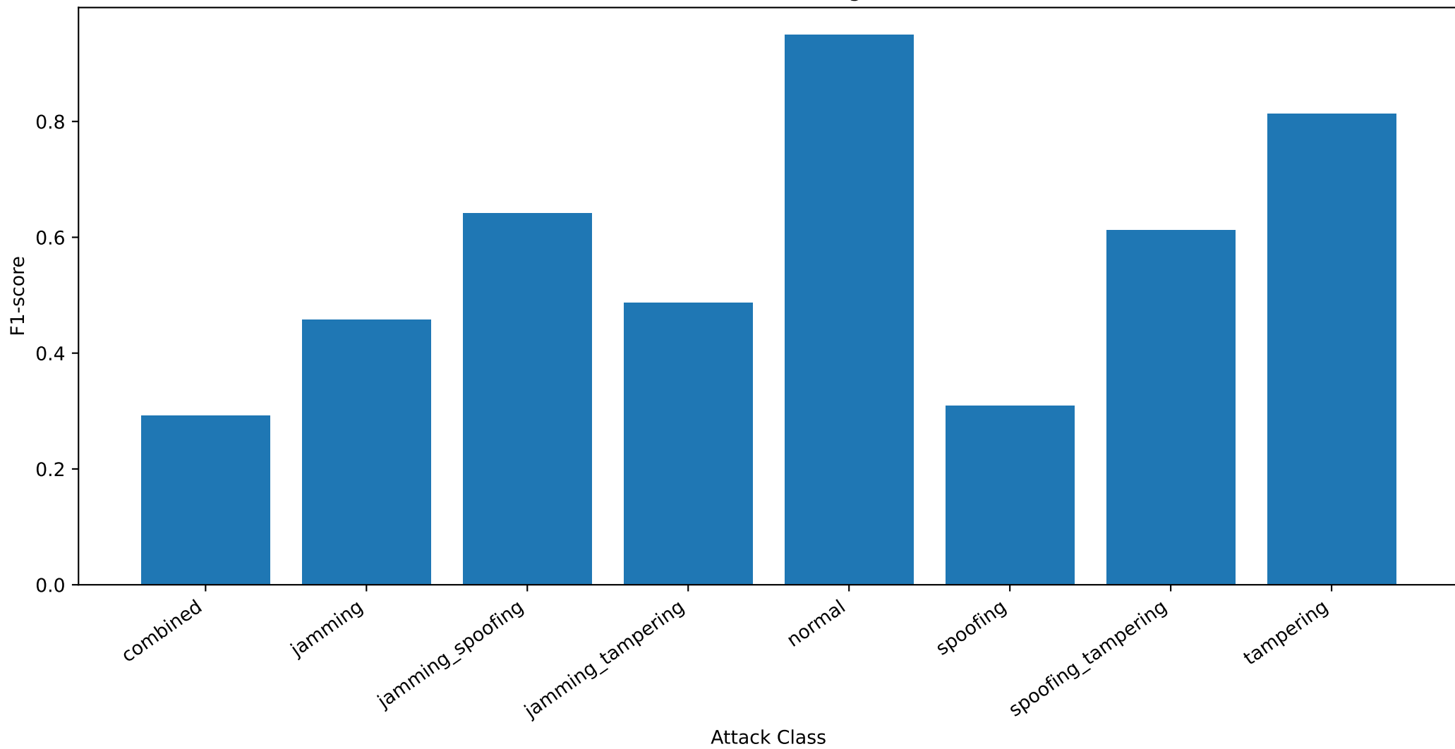
Per-Class F1-score for Weighted LSTM
