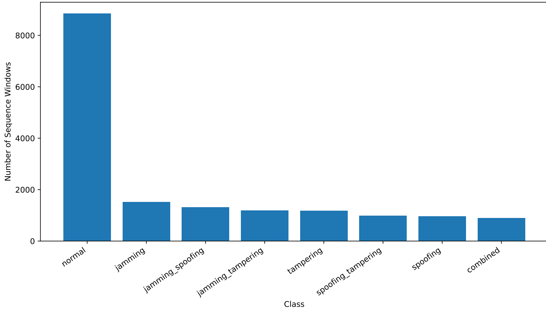
RA-MARS v3 Sequence Window Class Distribution
