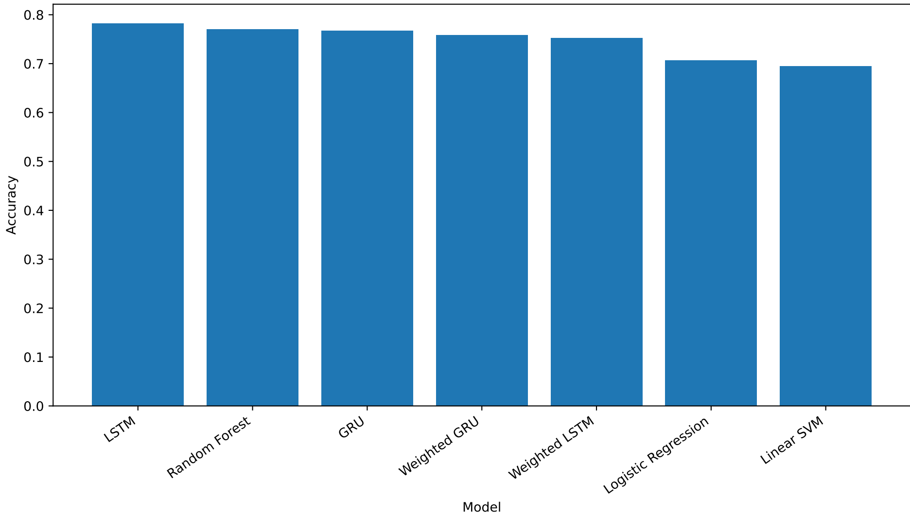
RA-MARS v3 Attack Detection Accuracy
