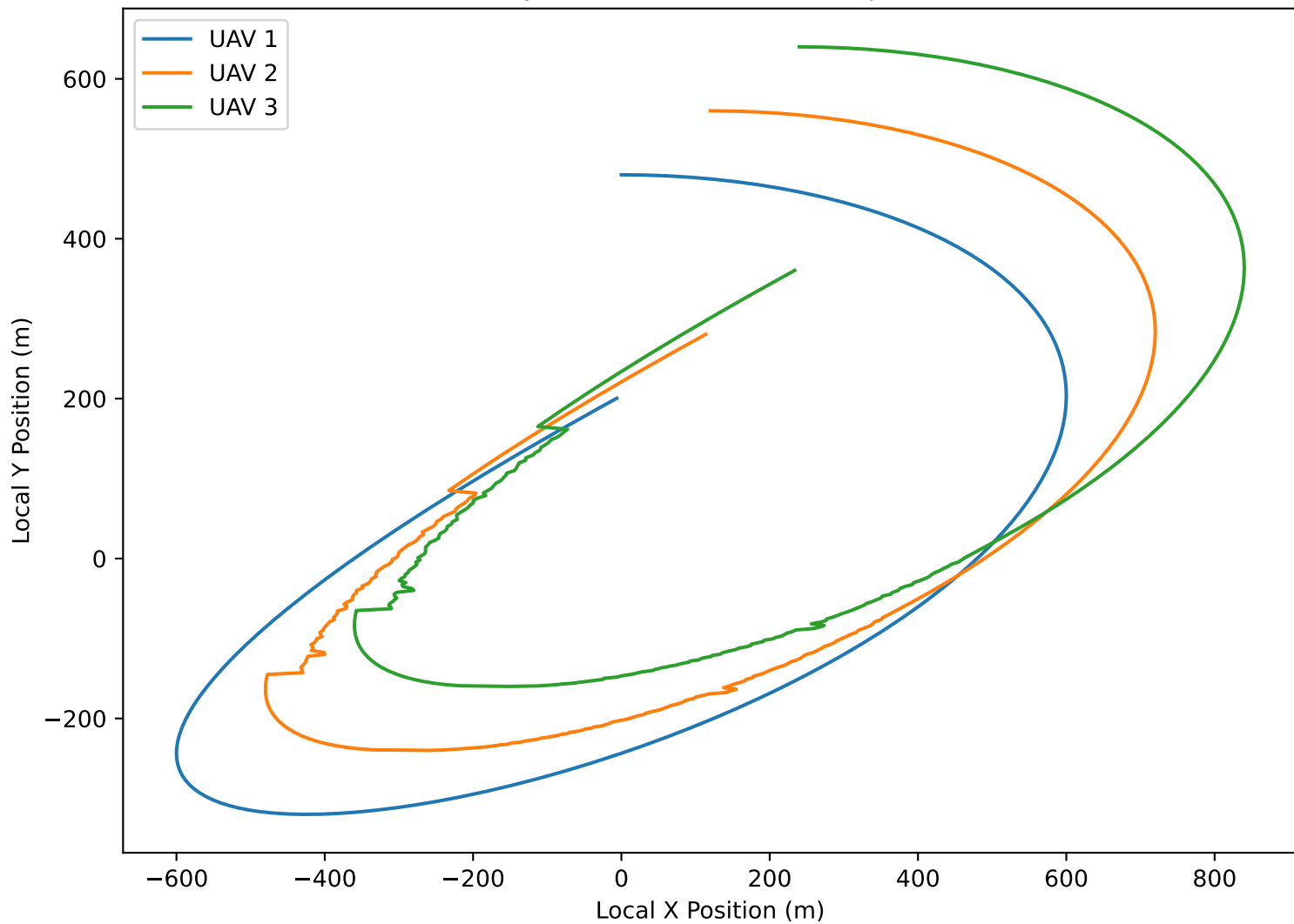
PX4-Style Multi-UAV Mission Trajectories
