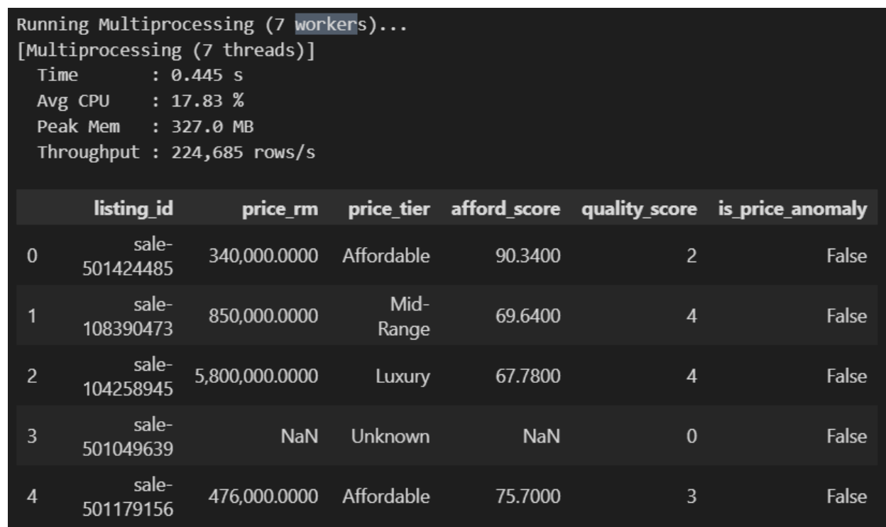
Figure 9.1: Multiprocessing Implementation Using ProcessPoolExecutor
