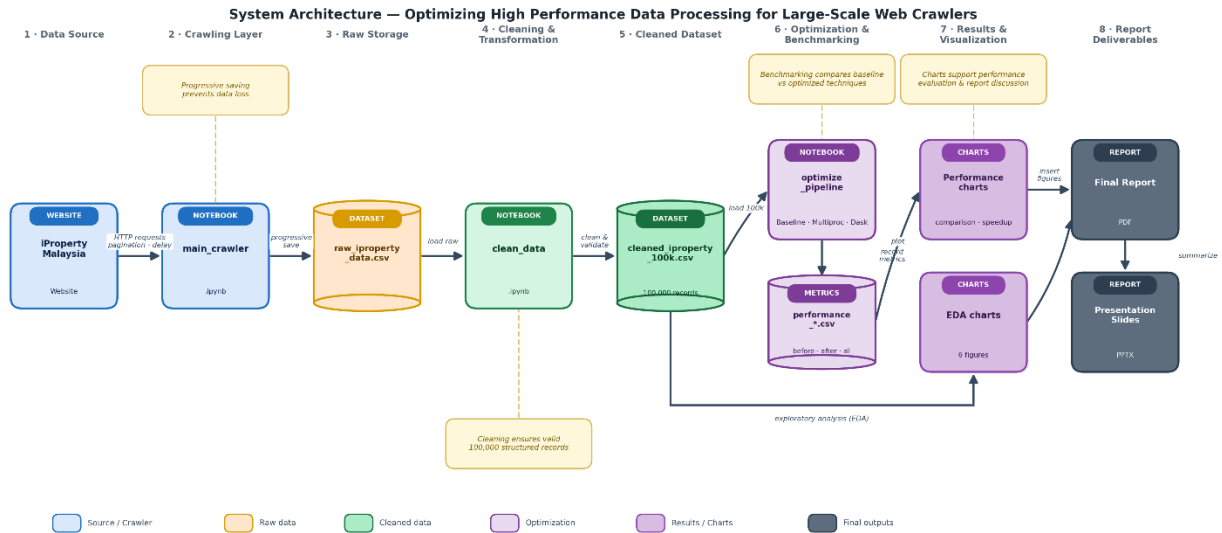
Figure 4.1: System Architecture of the iProperty Malaysia Data Processing Pipeline
