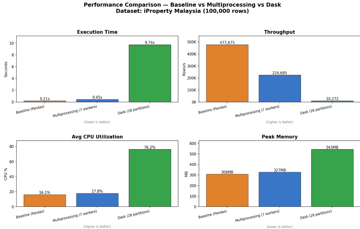
Figure 10.1: Performance Comparison Between Baseline, Multiprocessing, and Dask
