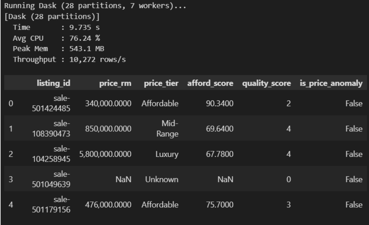
Figure 9.2: Dask Distributed-Style Processing Implementation
