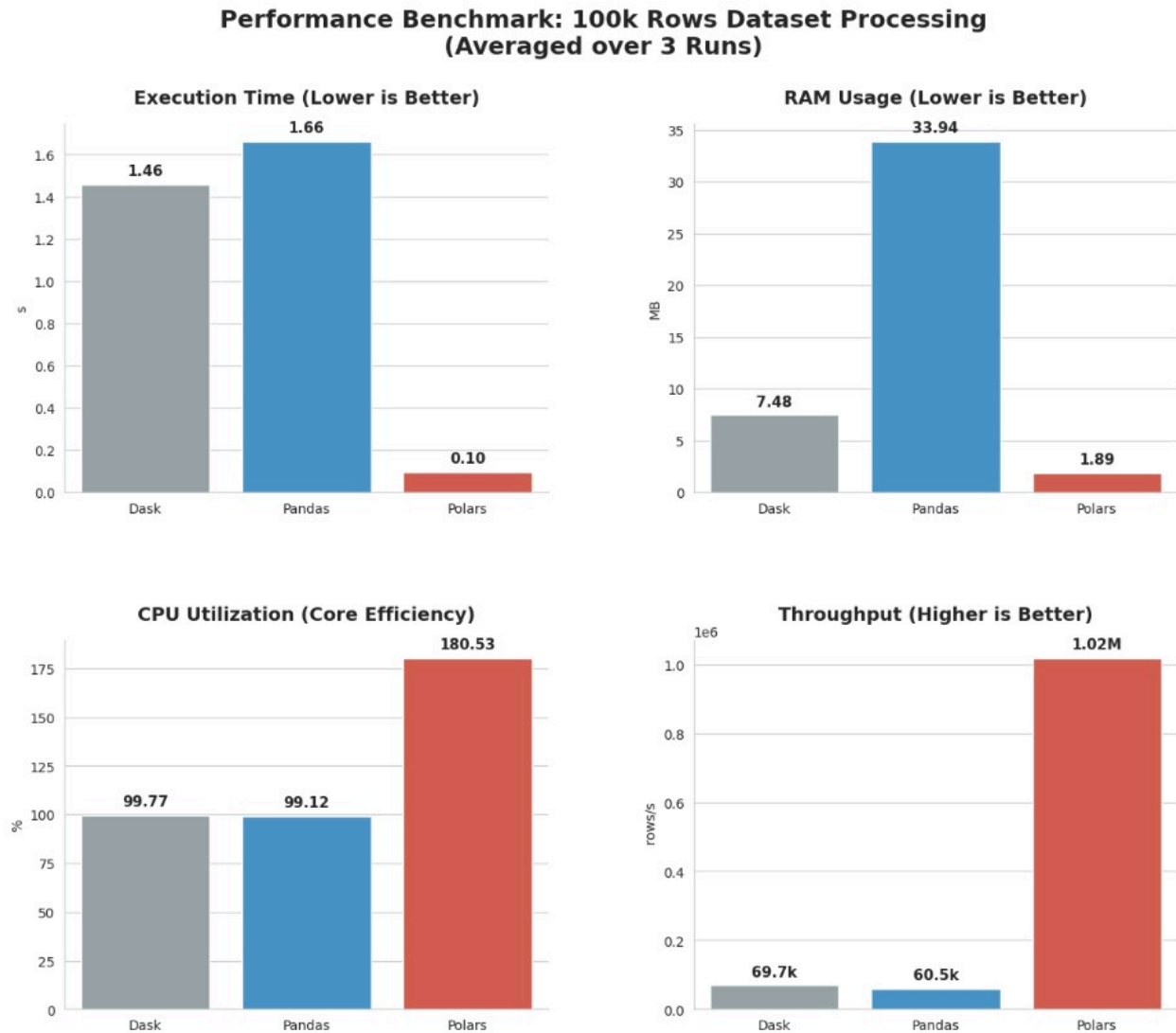
Figure 6.3 Comparison Performance Chart
