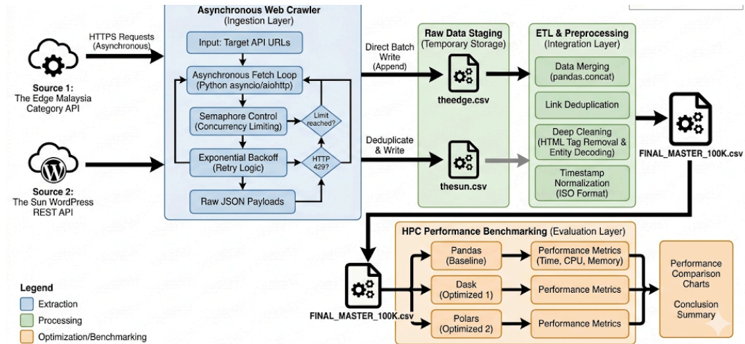
Figure 2.1 Architecture design of the web scraping and data preprocessing pipeline
